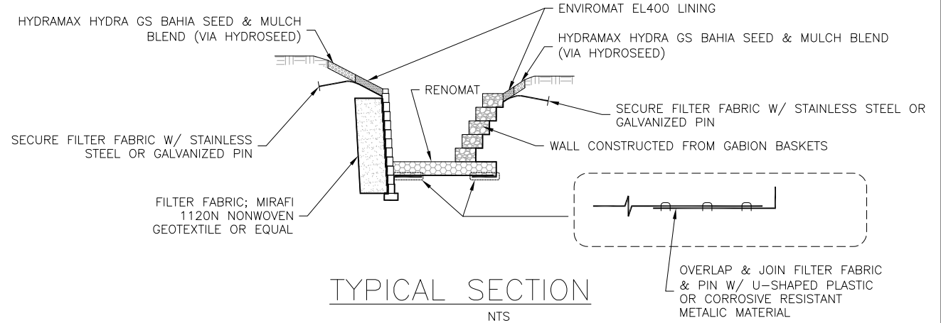
SLOPE STABILIZATION DETAIL (ENVIROMAT LINING)
