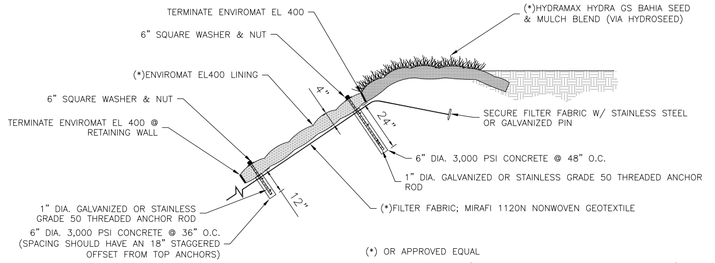
SLOPE STABILIZATION DETAIL (ENVIROMAT LINING)
