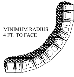
Anchor™ Diamond Pro Stone Cut™ Retaining Wall OUTSIDE CURVE DETAILS
