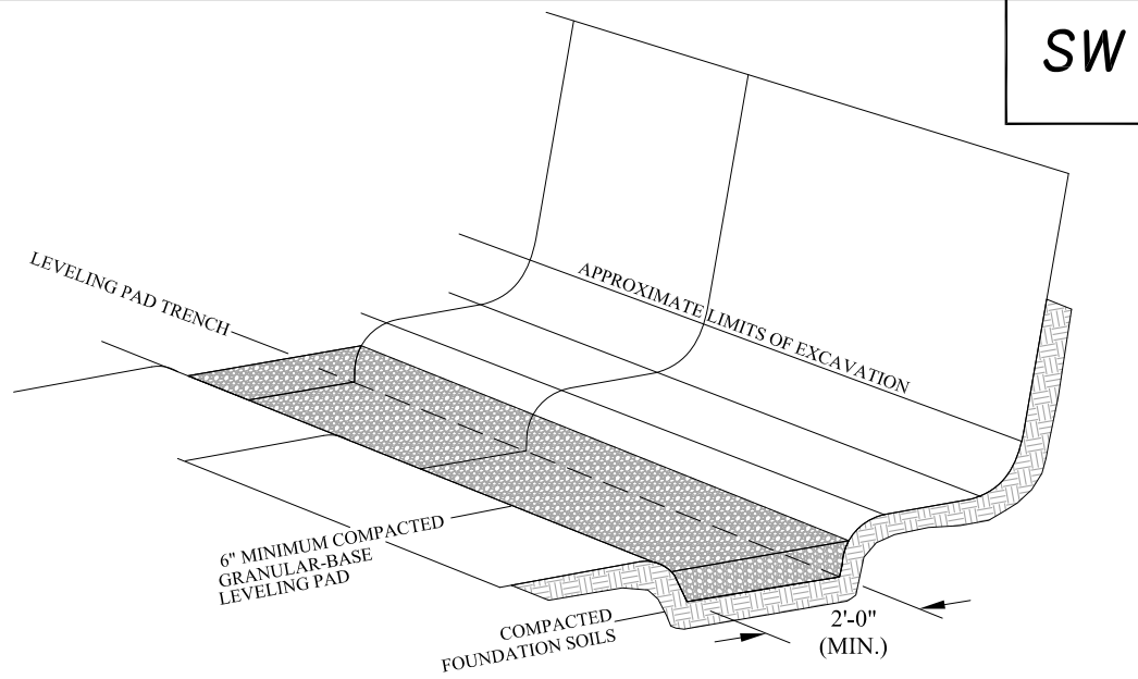
Anchor™ Diamond Pro Stone Cut™ Retaining Wall TYPICAL BASE PREPARATION (SCALE: NONE)
