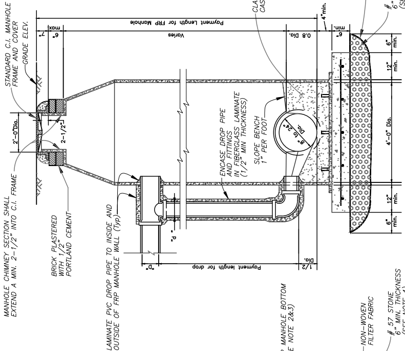
SECTION C-C
