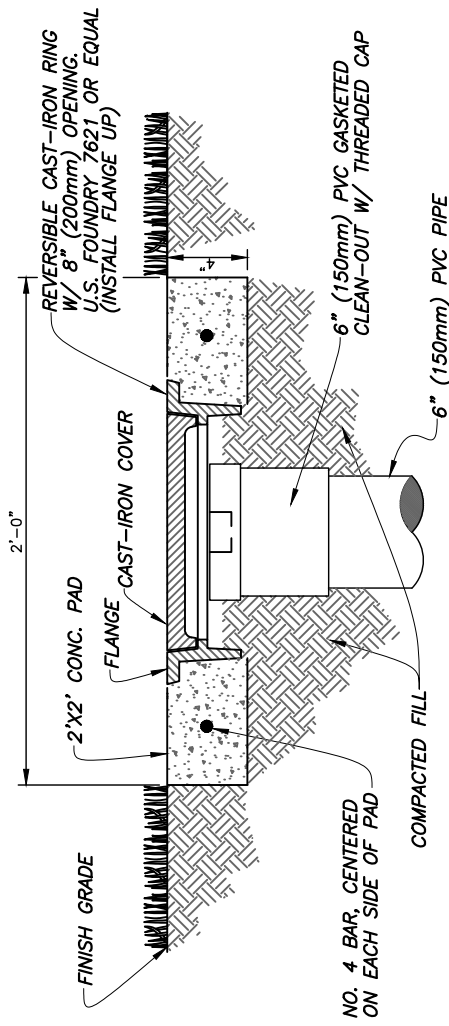
CLEAN-OUT W/COVER FOR GRASSED AREAS W/VEHICULAR TRAFFIC
