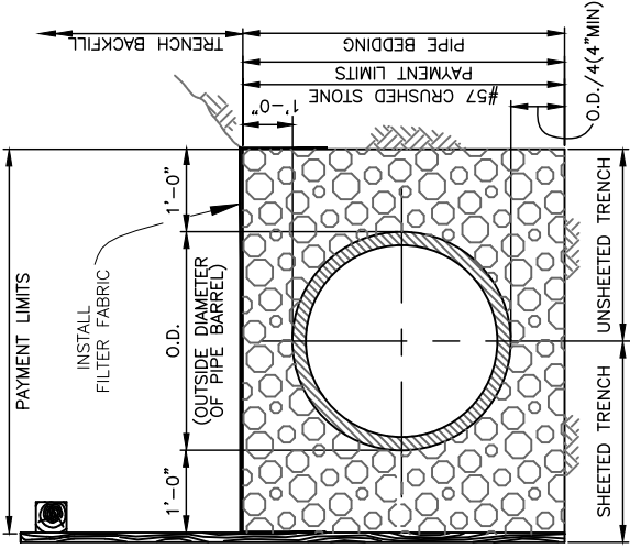
CLASS B-1 BEDDING
