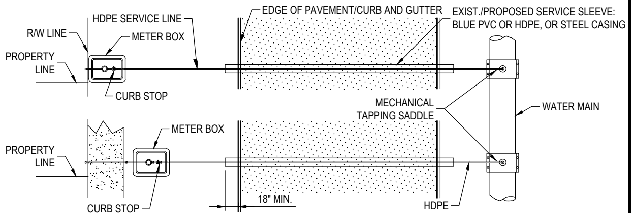
PLAN VIEW - SINGLE METER
