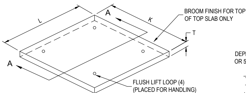
SLAB ISOMETRIC
