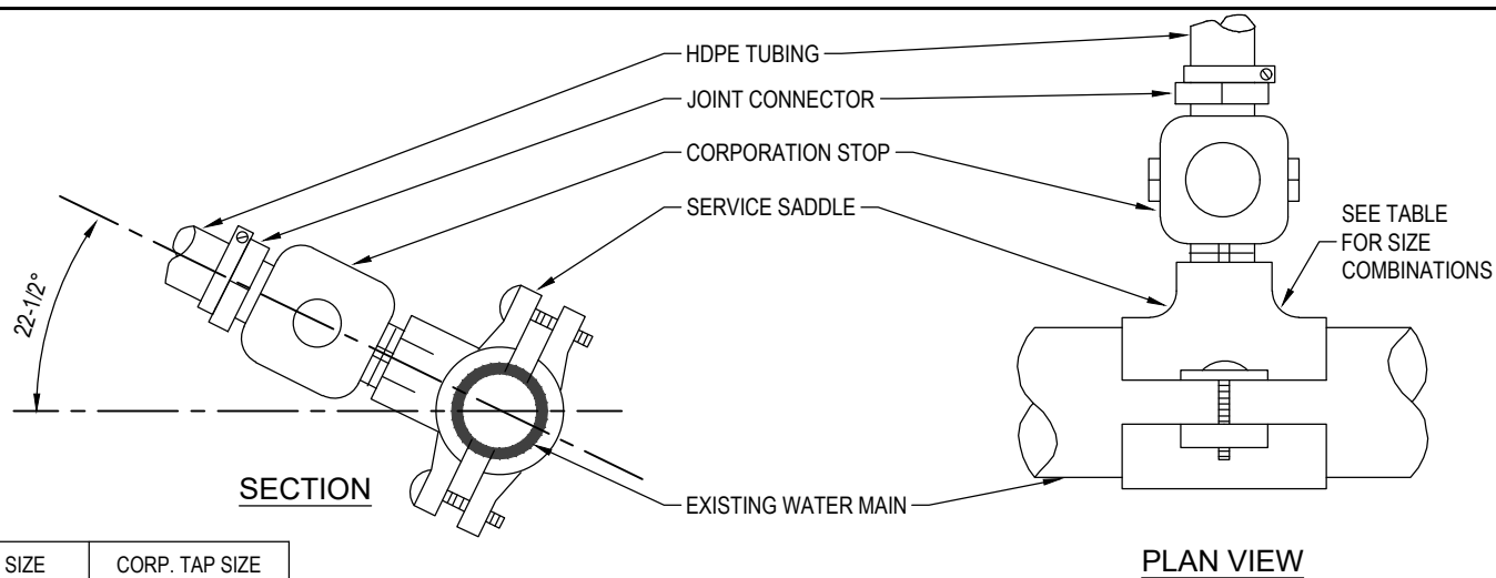
SADDLE TAP DETAIL
