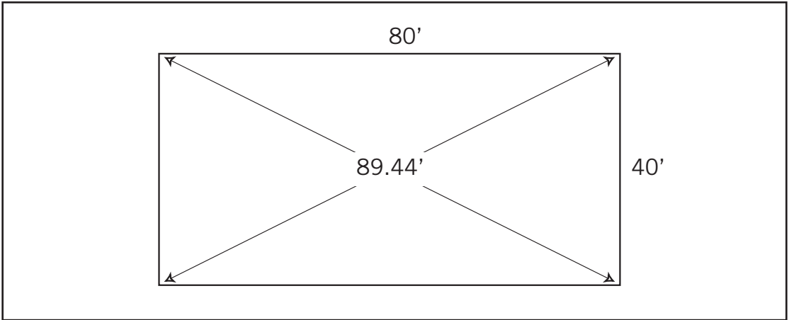
Figure 5. Determining the Length of the Diagonal
