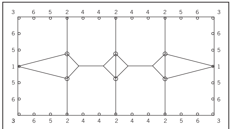
Figure 47. Tensile Tensioning, Example 1
