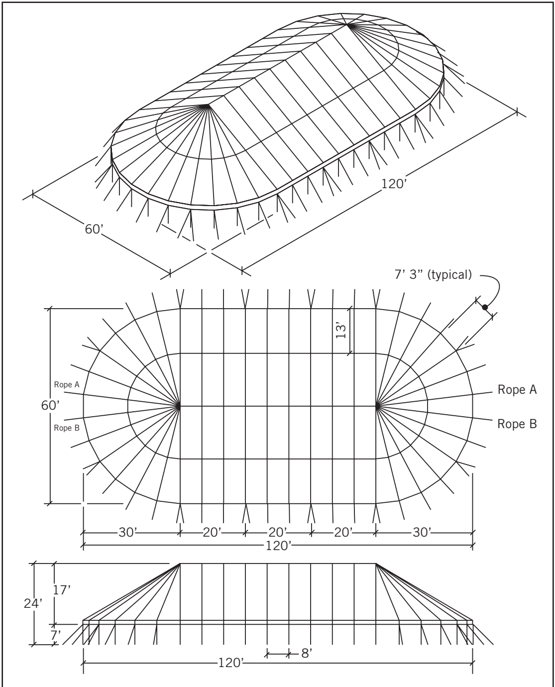
Figure 33. Tensioning a 60' x 120' Round-End Tent
