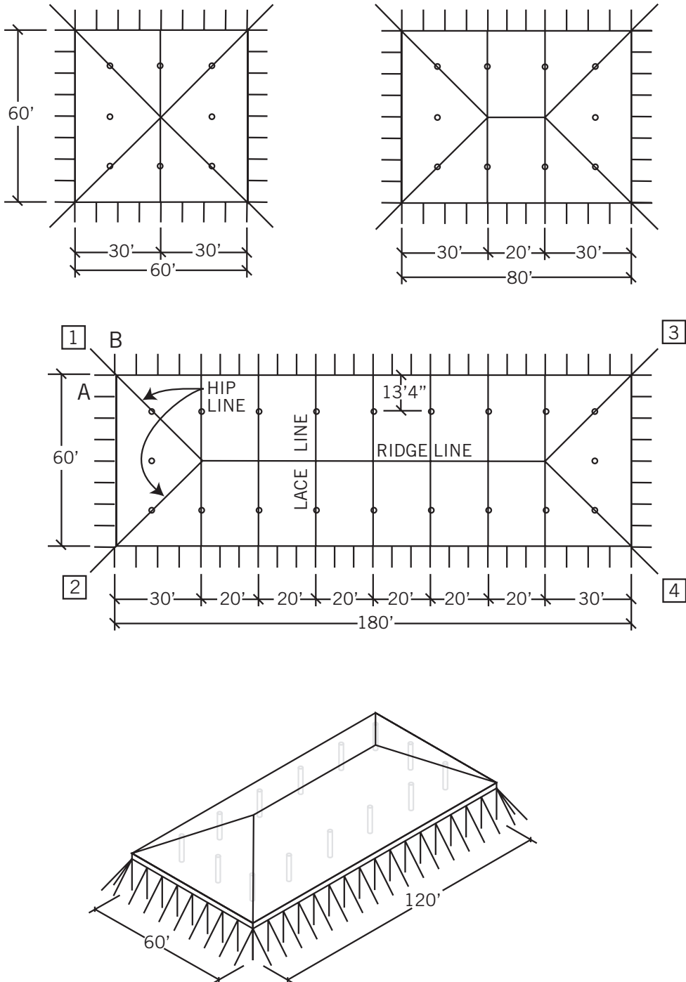
Figure 31. Tensioning a 60' x 120' Square-End Tent
