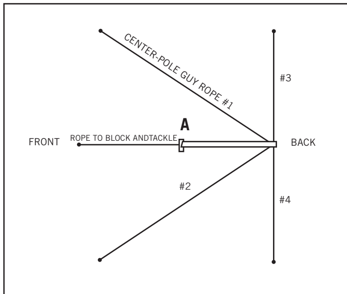
Figure 42. Center Pole and Guy Ropes Prior to Raising
