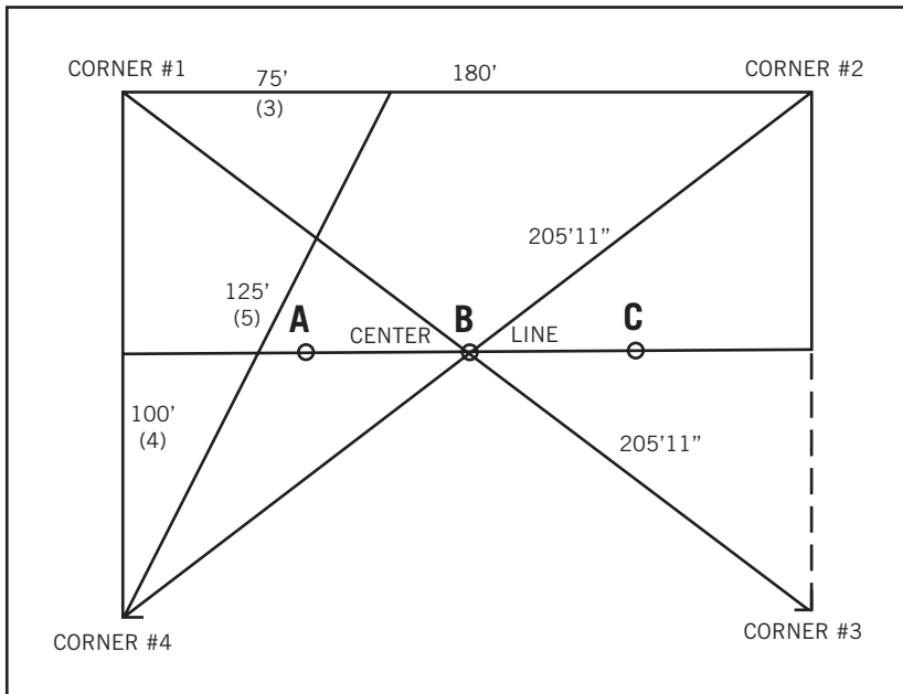
Figure 37. Perimeter Method of Layout with 3-4-5 Triangle 100' x 180' square-end bail-ring tent
