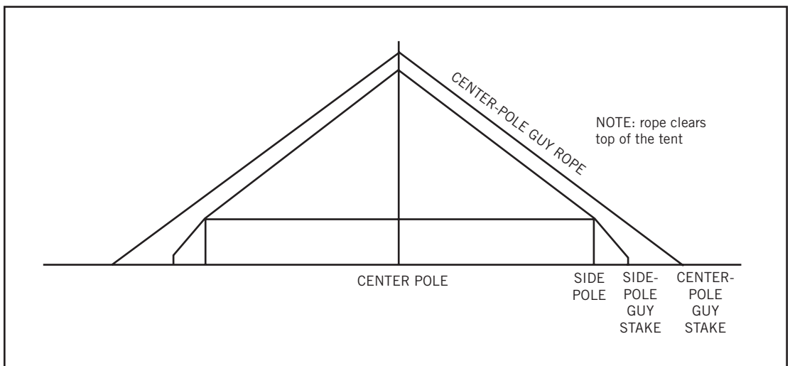
Figure 39. Tent with Center-Pole Guy Ropes—End View
