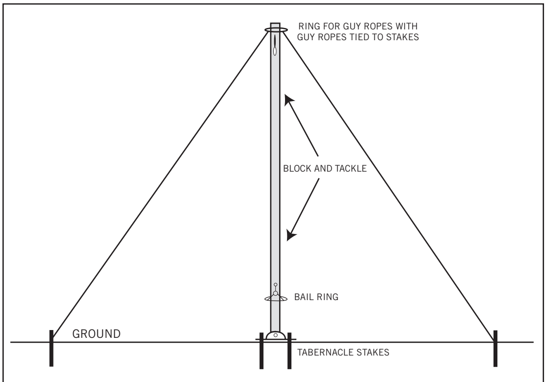
Figure 43. Center Pole Raised with Bail Ring in Lowered Position
