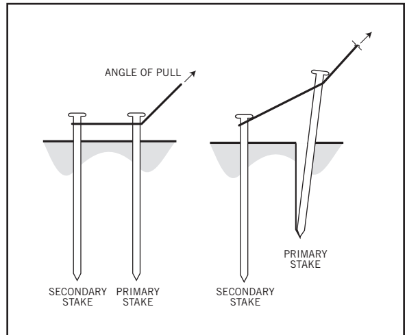
Figure 17. Double Staking
