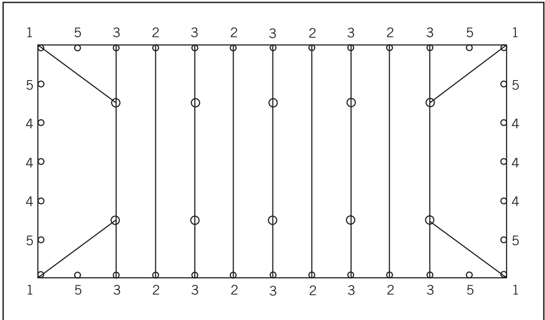
Figure 48. Tensile Tensioning, Example 2
