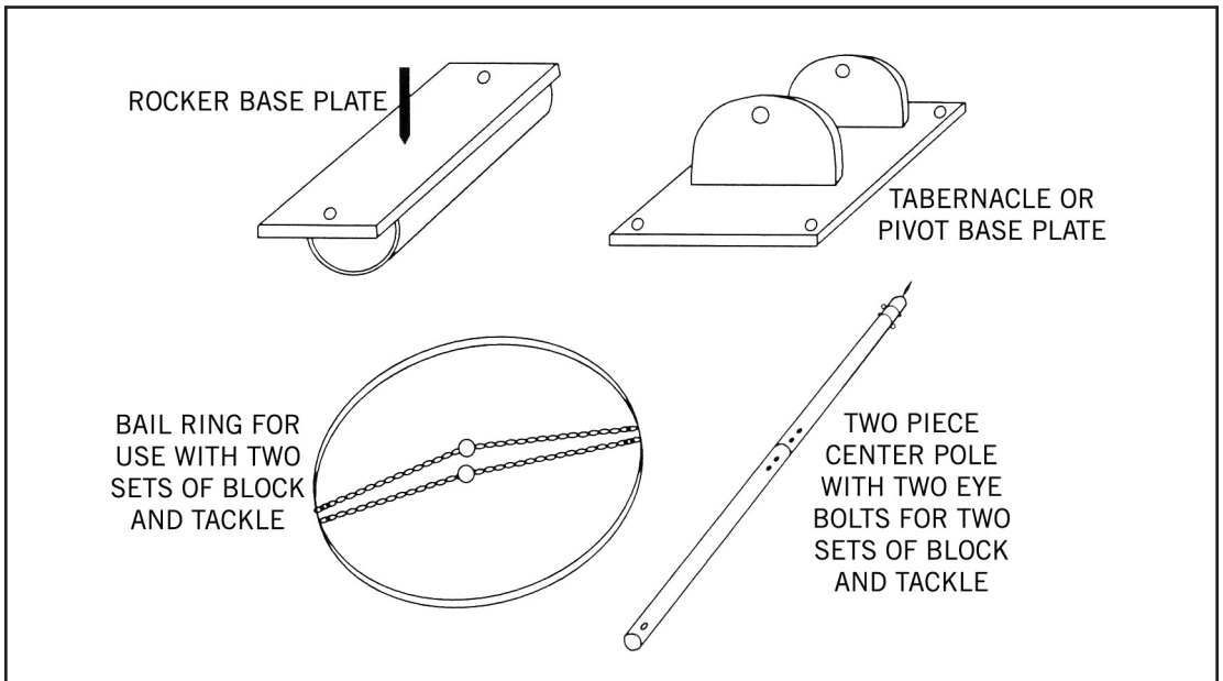
Figure 40. Typical Bail-ring Tent Hardware Parts
