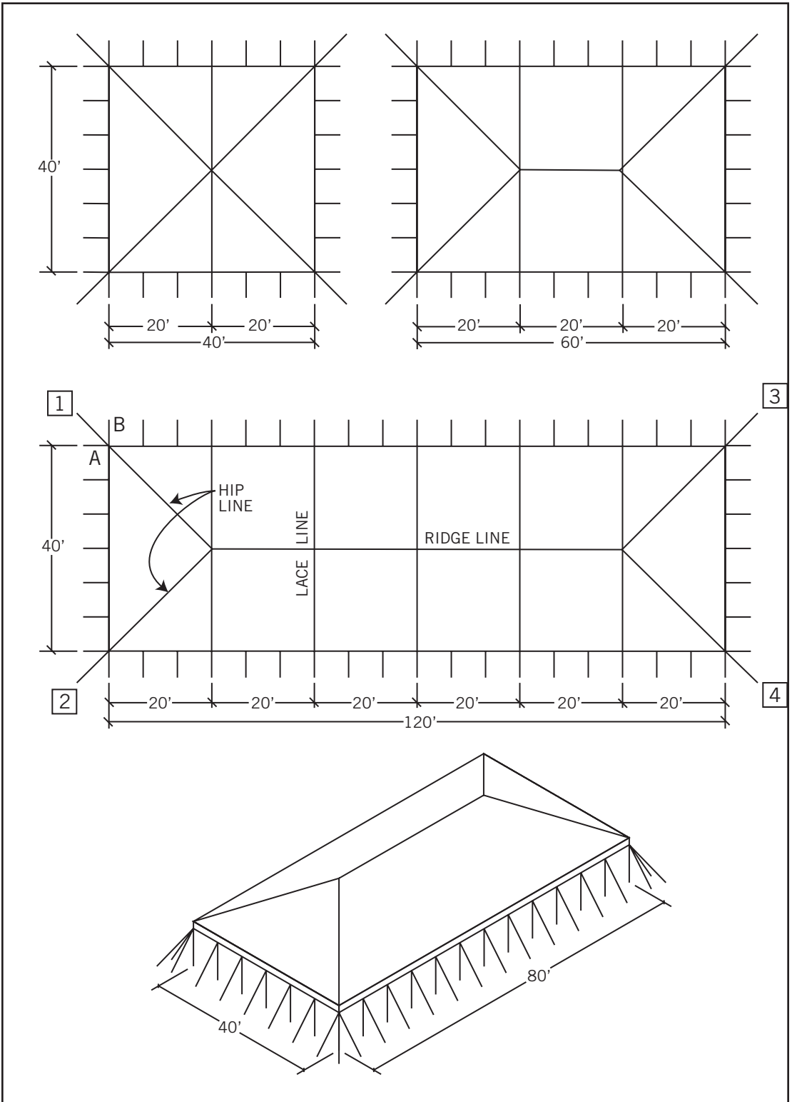
Figure 30. Tensioning a 40' x 80' Square-End Tent
