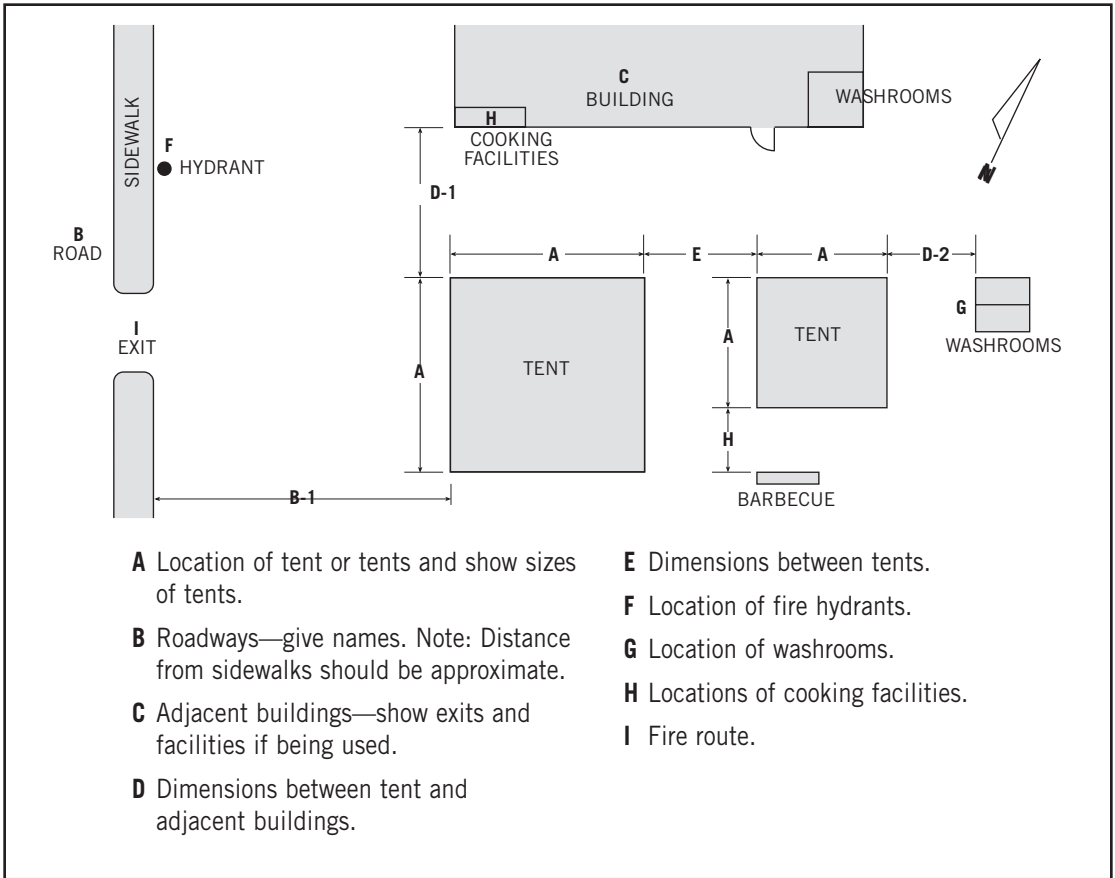
Figure 2. Site Plan to Scale
