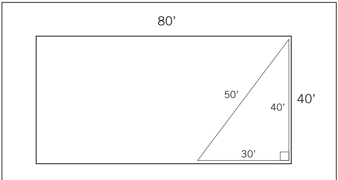
Figure 7a. Squaring a Tent Using the 3-4-5 Method
