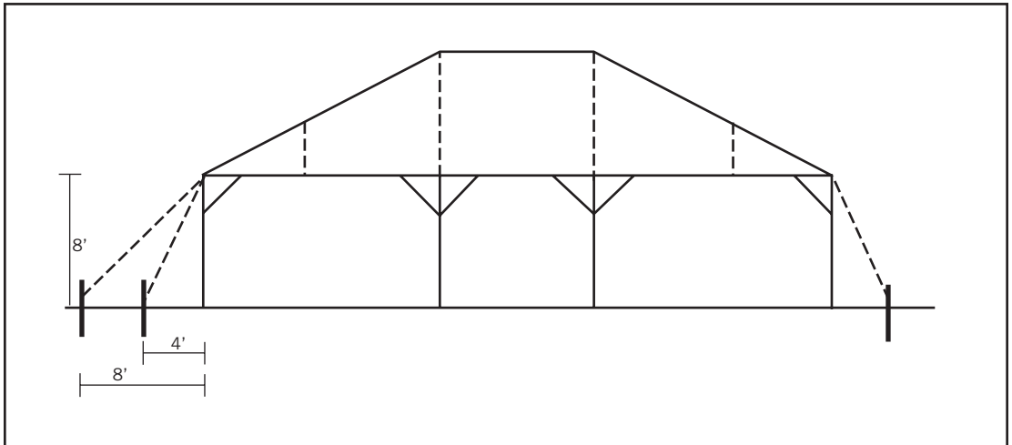
Figure 45. Suggested Guy-Rope Angle for Typical Frame Tent
