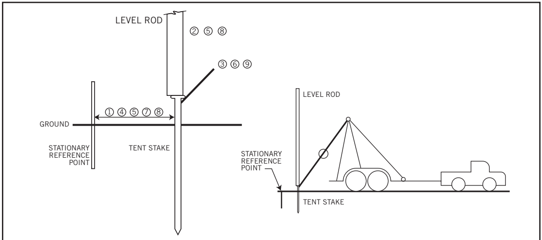
Figure 21. Field Test Setup
