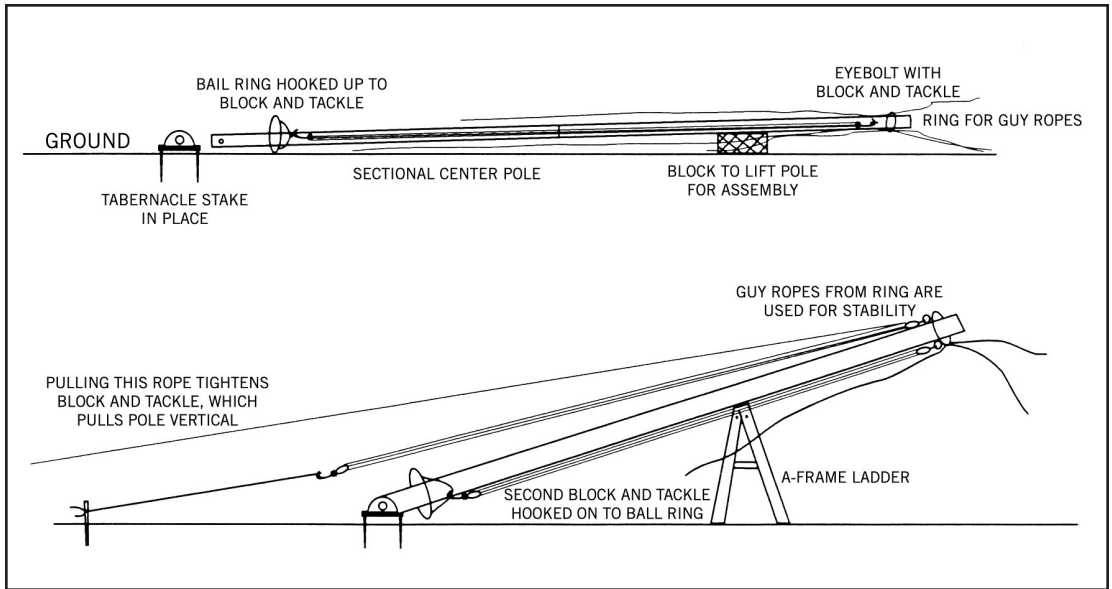
Figure 41. Ground Assembly of Center Pole and Related Equipment
