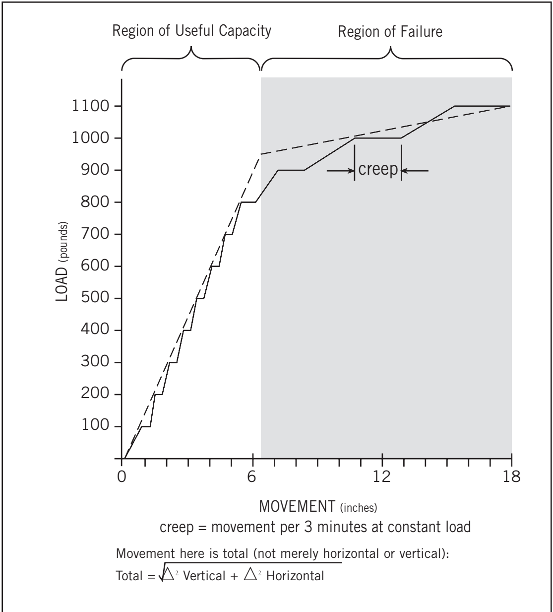
Figure 25. Stress vs. Strain Graph for Stake Pull Test
