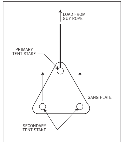
Figure 19. Gang Staking
