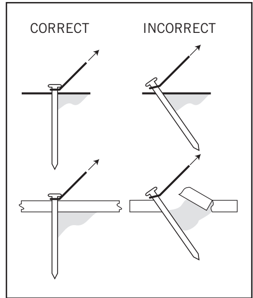
Figure 13. Stake Driving Angle
