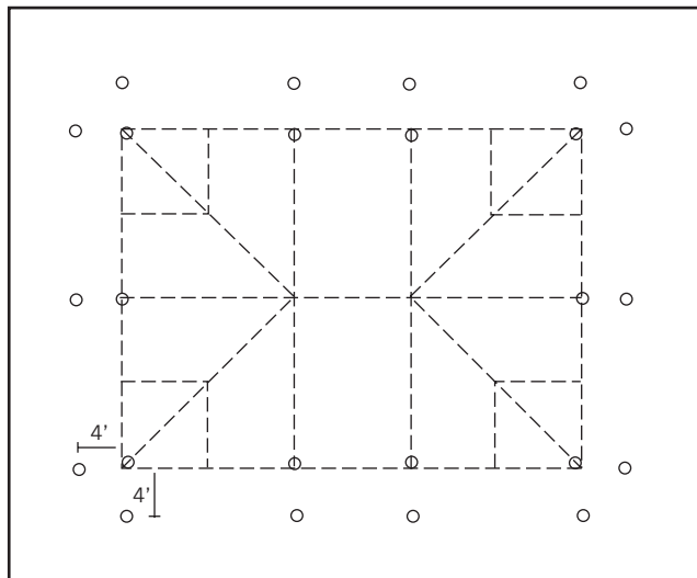
Figure 44. Suggested Stake Placement for Typical Frame Tent
