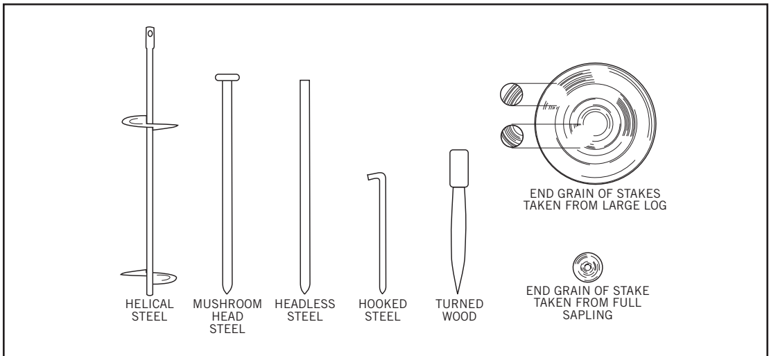
Figure 16. Various Tent Stakes
