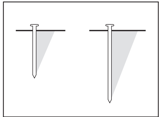
Figure 11. Soil Wedge Size and Sideways Resistance
