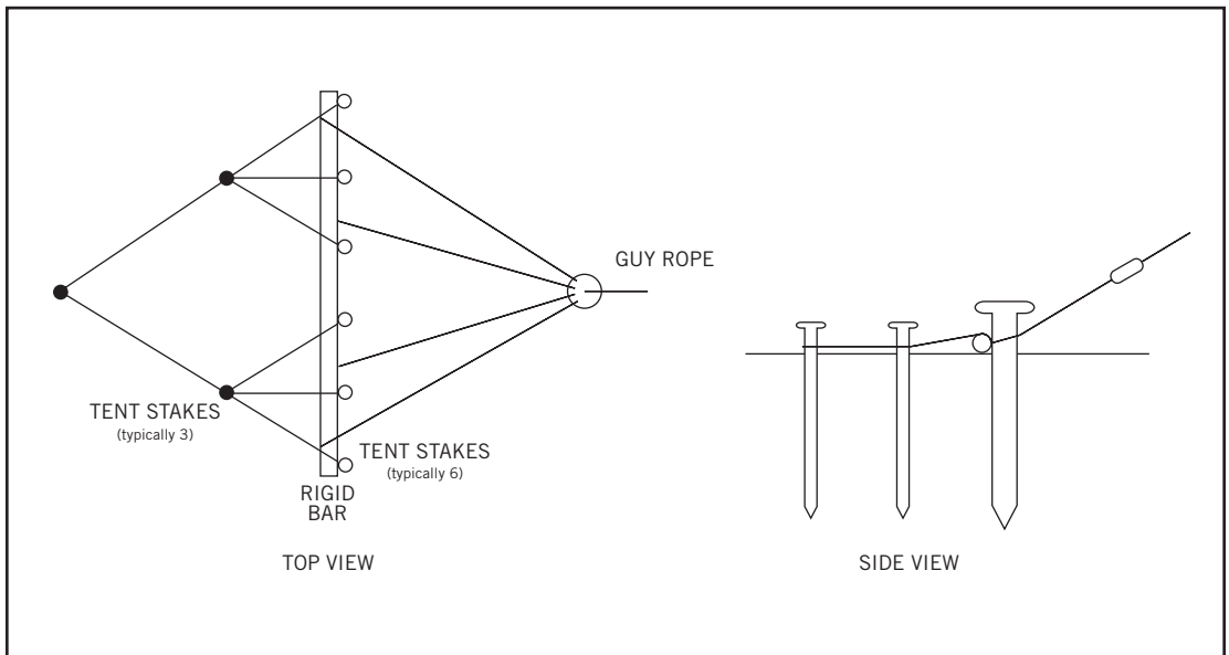
Figure 20. Buckle's Frog's Foot
