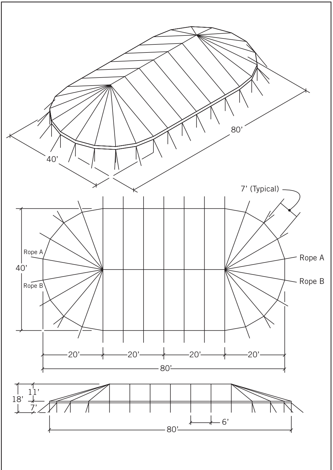
Figure 32. Tensioning a 40' x 80' Round-End Tent
