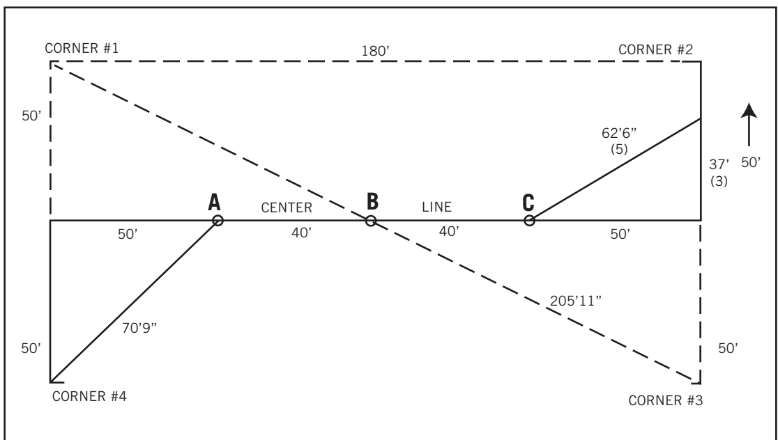
Figure 36. Center Line Method of Layout 100' x 180' square-end bail-ring tent
