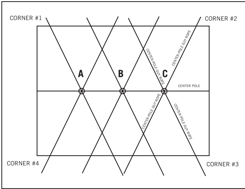
Figure 38. Staking Pattern for Center-Pole Guy Ropes
