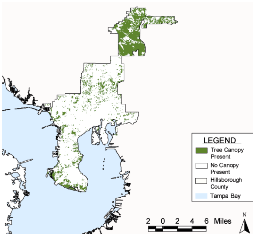
Figure 5. NDVI Results from 1985 Satellite Image
