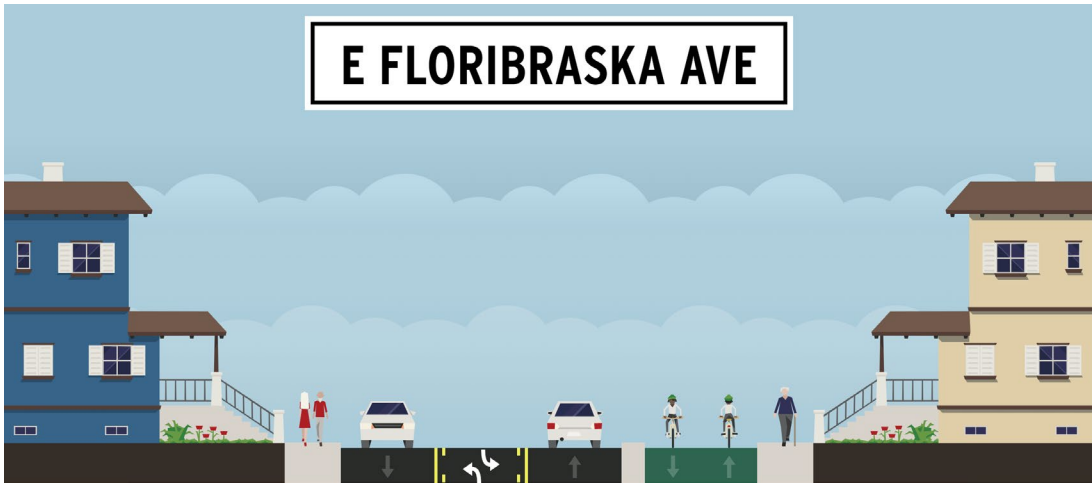
Graphic of the proposed improvements cross section displaying pedestrian, vehicle and bike lanes.
