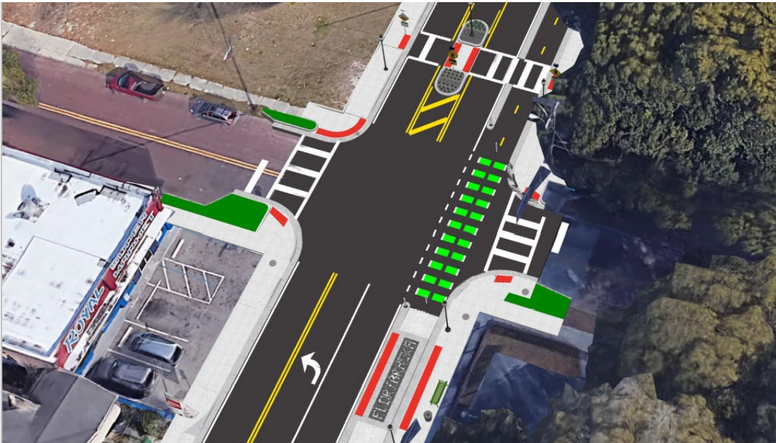
Aerial view of the proposed improvements near North Central Avenue displaying cross walks, bike lanes and curb ramps.
