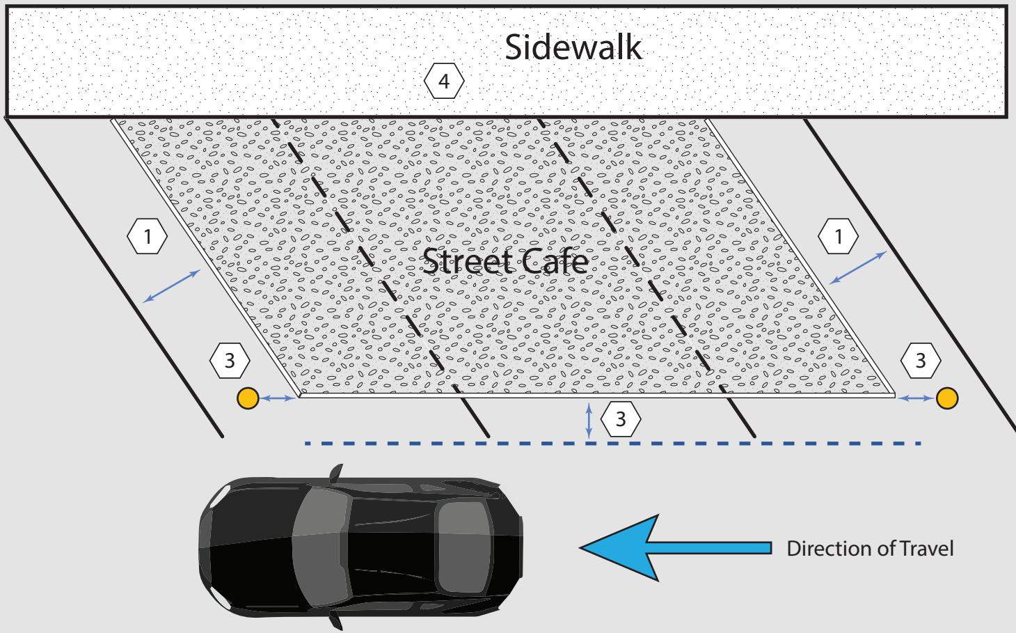
Design and Street Cafe Placement Angle Parking
