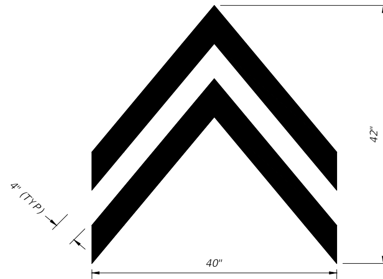
STANDARD SHARROW LINES
