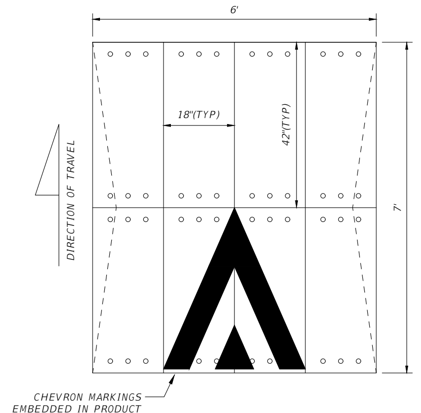
TRAFFICLOGIX - SPEED CUSHION (SC-070603-M) DETAIL
