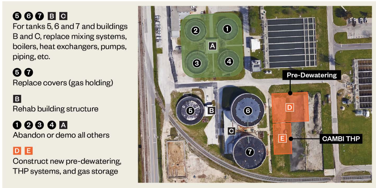
Figure 11.3-9: Site Plan – Proposed THP Facilities
