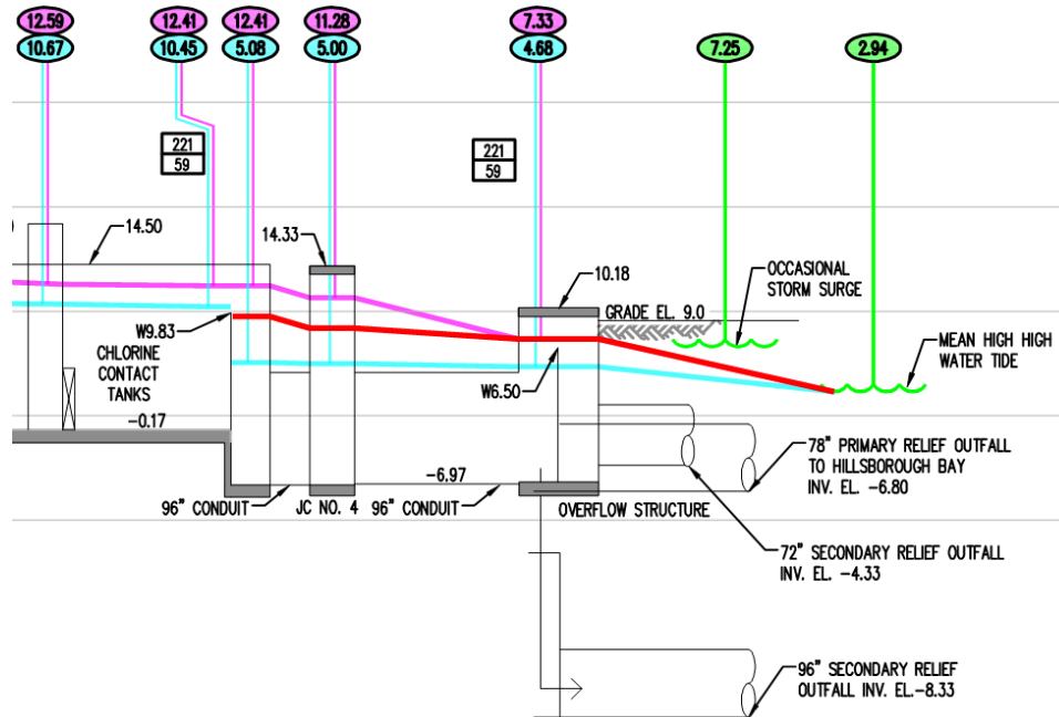
Figure 9.6-5: Second 96-inch Pipe Between JC 4 and Overflow Structure Hydraulic Improvements
