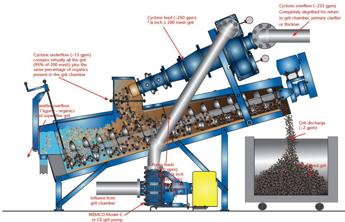
Figure 5.4-3: Picture of WEMCO Hydrogritter®
