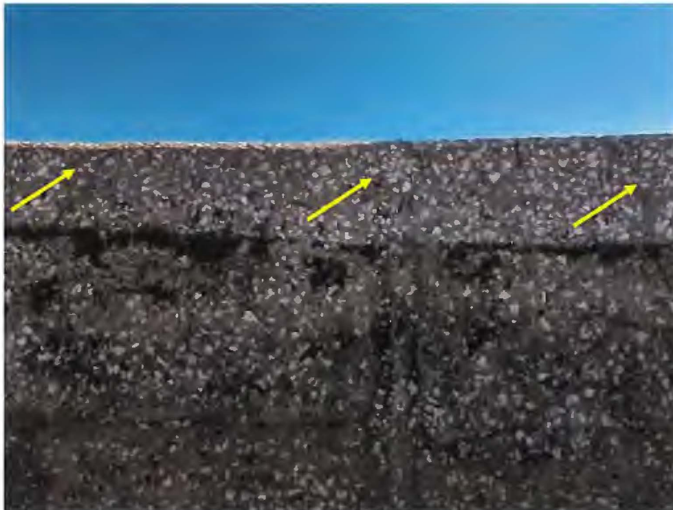
Photo 8 – Close-up of area shown in Photo 7.
