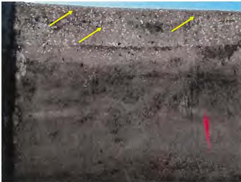
Photo 20 – Northwest wall of tank with vertical cracks.
