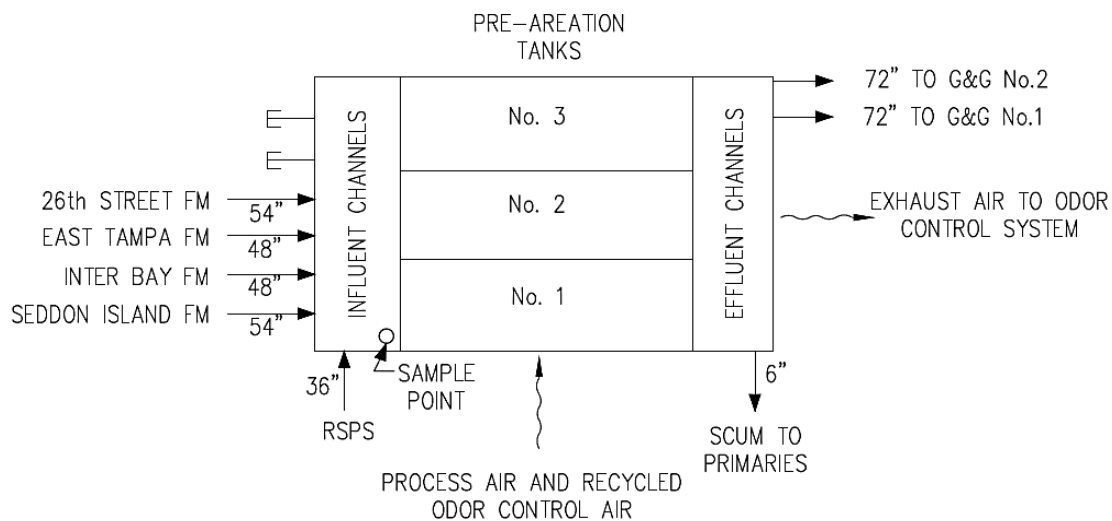
Figure 5.1-2: Junction Chamber No. 1 Flow Diagram
