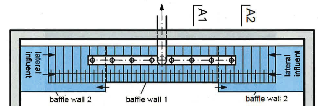
View of the Top of the DEMON Reactor
