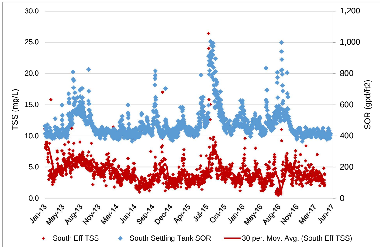
Figure 7.2-3: South Sedimentation Tank Performance at Peak SORs
