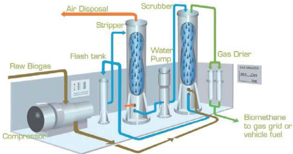
Figure 12.4-6: Typical Water Scrubbing Process Flow Diagram (Courtesy of Greenlane)
