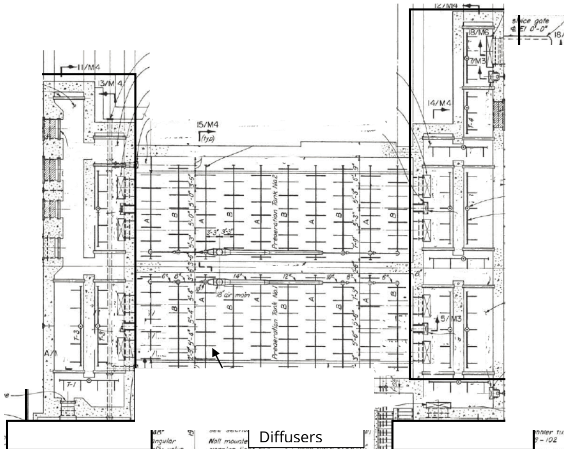
Figure 5.1-3: Record Drawing of Junction Chamber No. 1 (Not Including Tank No. 3)
