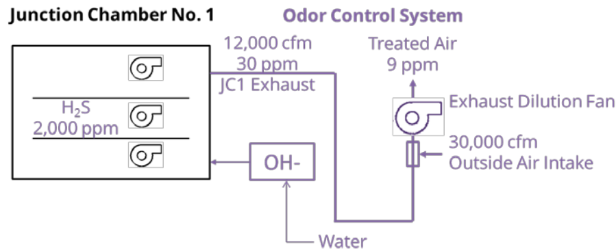
Figure 5.2-11: Flow Diagram of Alternative 4 Hydroxyl Radical (OH-) Oxidation
