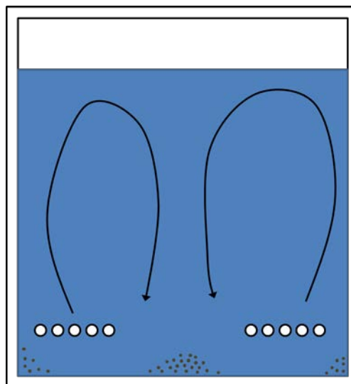
Figure 5.1-4: Pre-Aeration Tank Cross Section Showing Rotational Mixing Pattern
