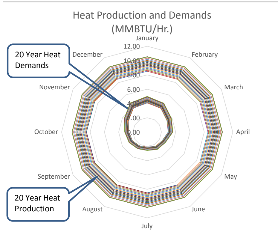
Figure 12.4-3: CHP Heating Demands and Production (Optimize Existing Liquid Stream, (Acid Gas Biosolids))
