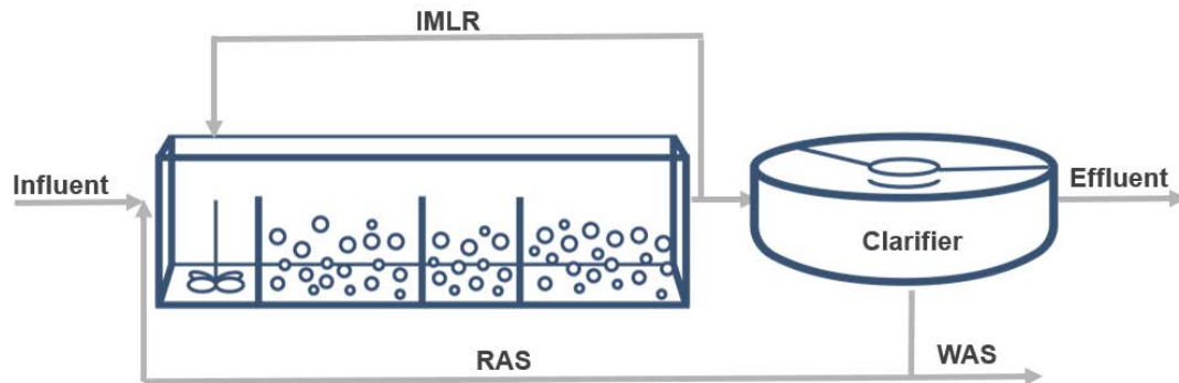
Figure 7.1-2: Separate Stage Denitrification
