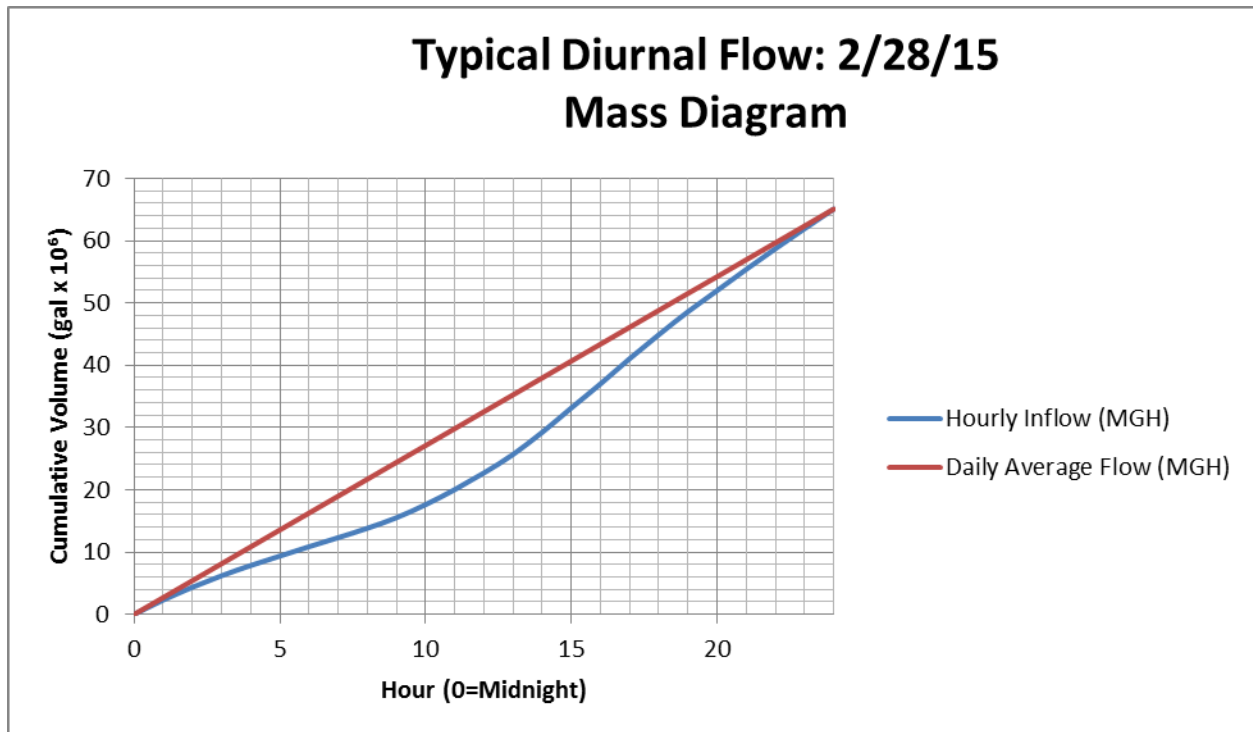
Figure 4.2-1: February 28, 2015 Mass Diagram
