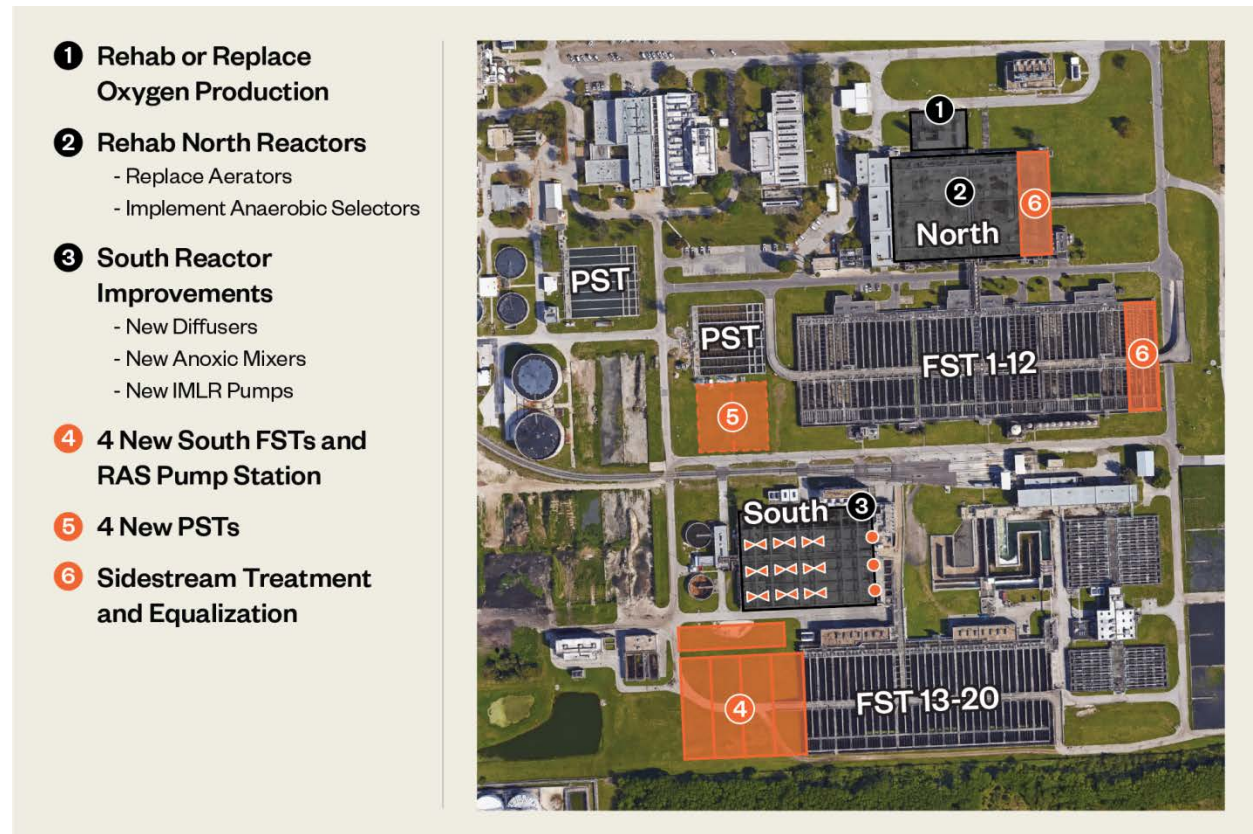
Figure 7.5-1: Selected Alternative: Optimize Existing
