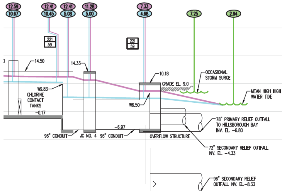
Figure 9.6-2: Existing CCT Surcharging at Peak Hourly Flow
