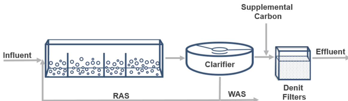
Figure 7.1-3: Modified Ludzack Ettinger (MLE)
