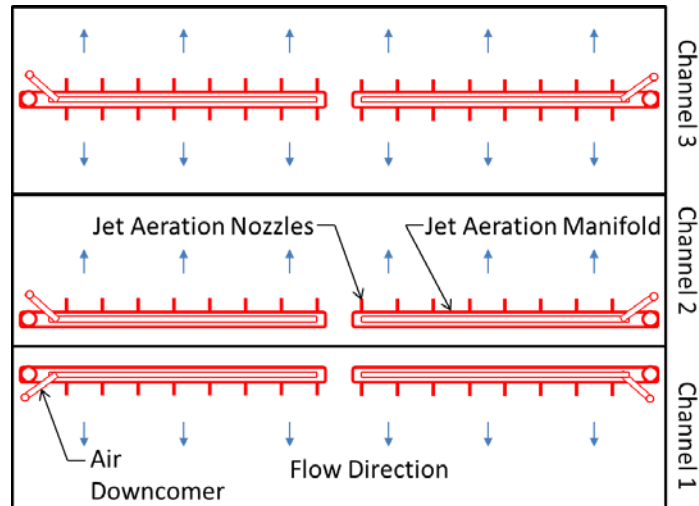
Figure 5.1-6: Proposed Layout for Alternative 3
