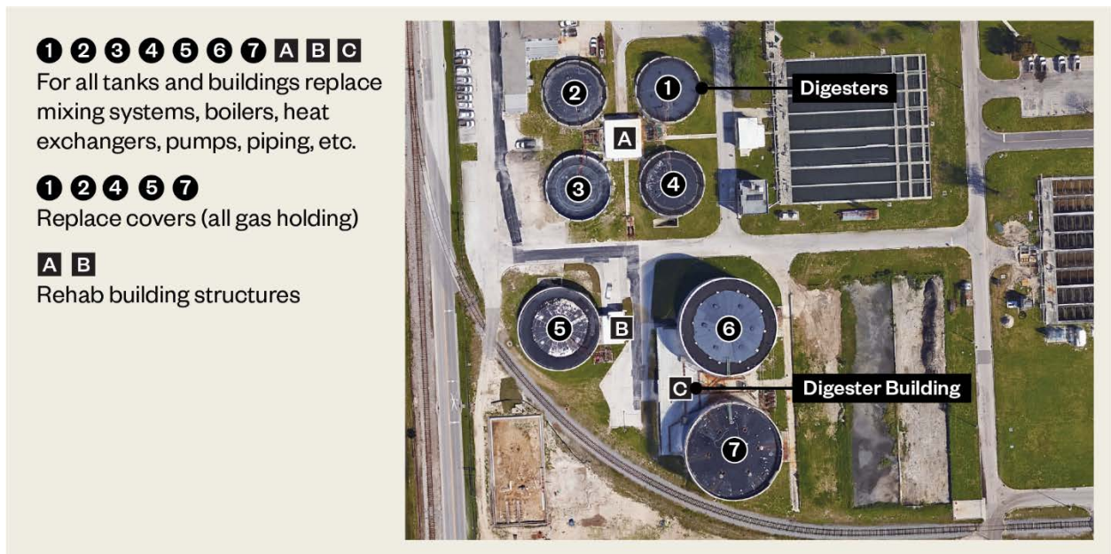
Figure 11.3-2: Site Plan – Existing HFC AWTP Solids Processing Facilities Improvements
