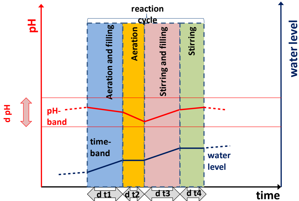
Figure 10.3-2: Process Control Strategy for DEMON® SBR Process (Courtesy of World Water Works)
