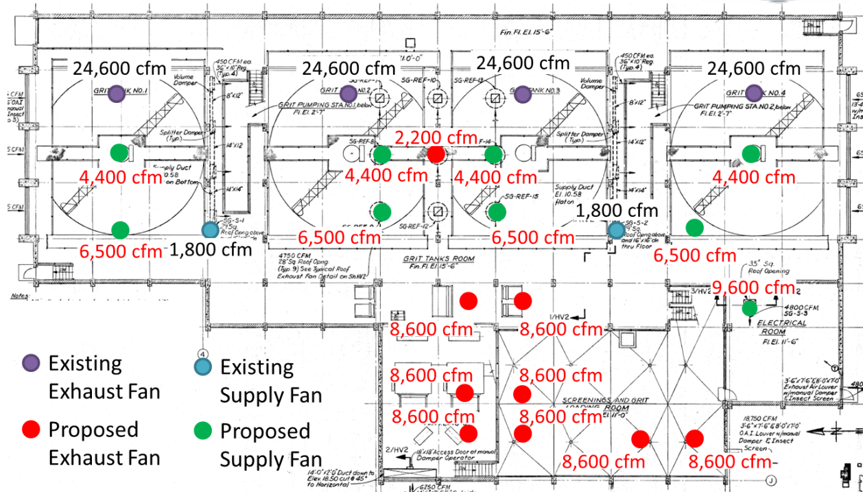
Figure 5.3-4: S&G Building No. 2 Fan Improvements to Increase Ventilation
