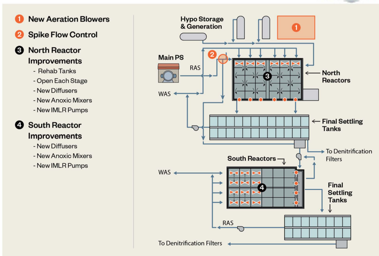
Figure 7.4-3: Summary of Capital Improvements Req. for Alternative 2D- MLE In Parallel (Diffused Air)
