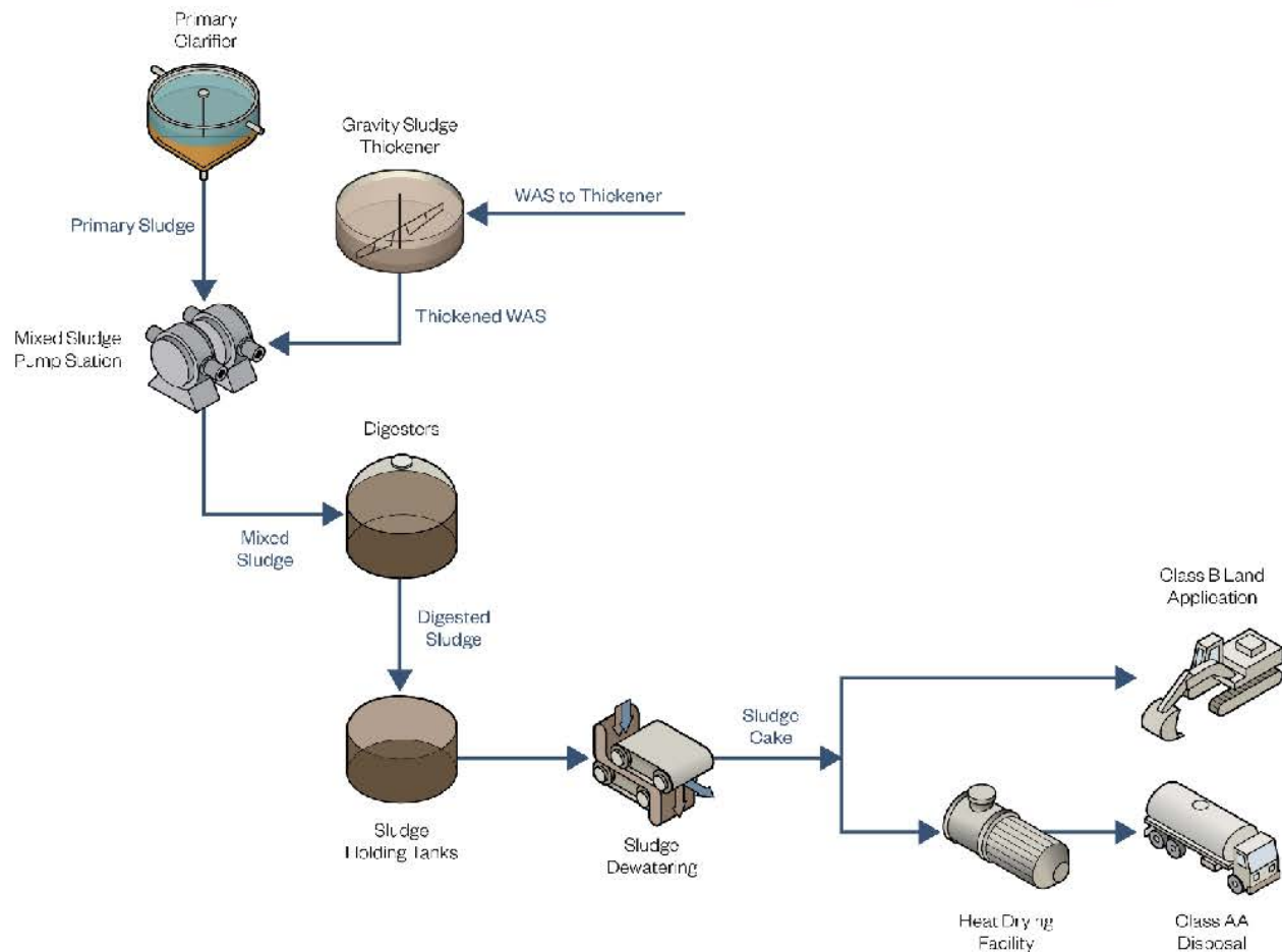
Figure 11.1-1: Existing HFC AWTP Process Schematic
