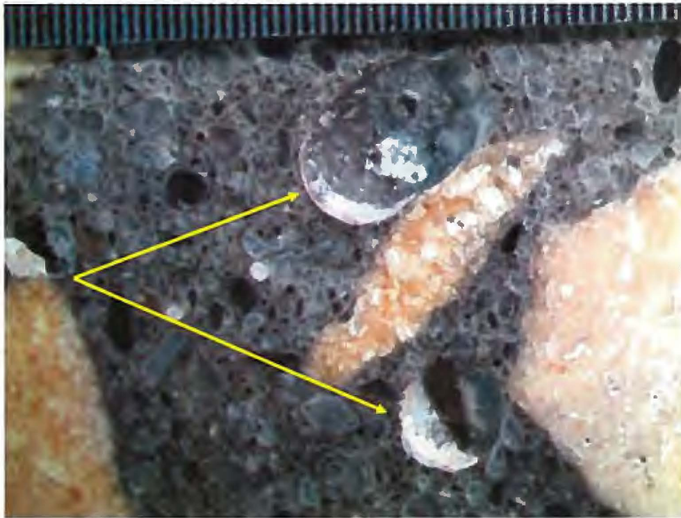
Photo 8 – Magnified view of entrapped air void. Scale = 0.01 inches
