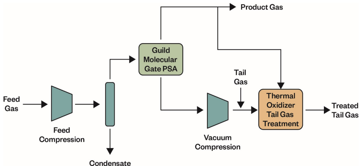
Figure 12.4-4: Typical PSA Process Flow Diagram (Guild Associates Molecular Gate™ Example)
