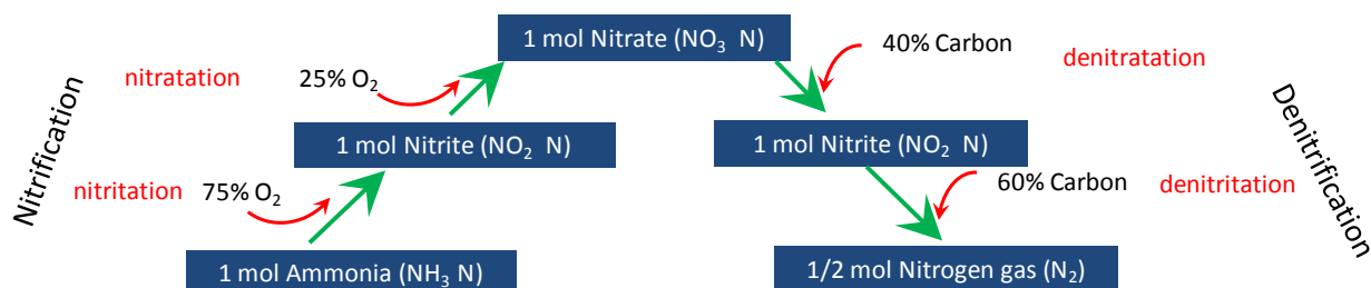
Figure 10.2-1: Nitrification and Denitrification Pathway for Nitrogen Removal
