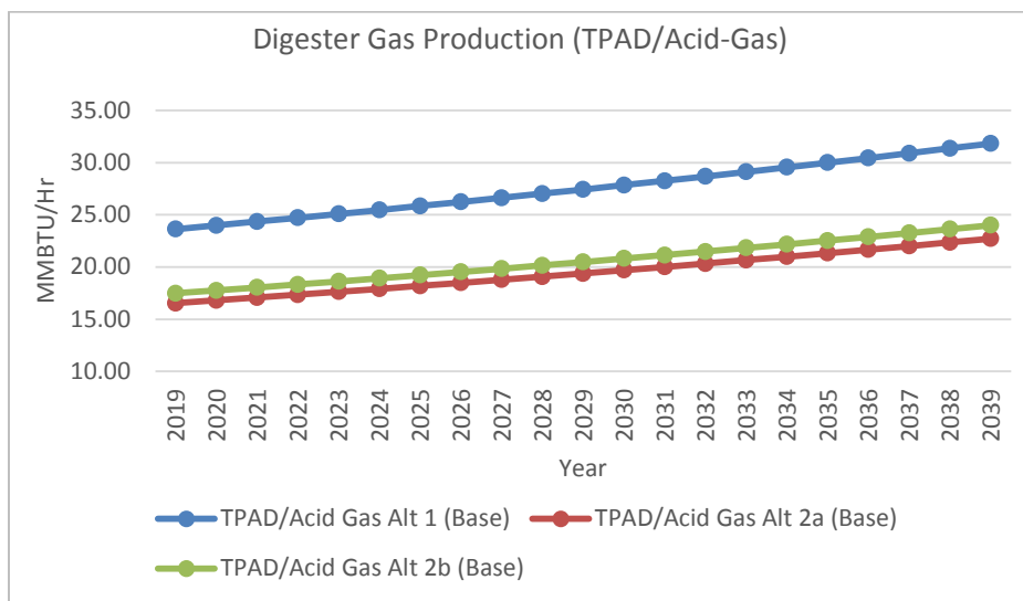
Figure 12.3-2: TPAD/Acid Gas Biosolids Treatment Digester Gas Production
