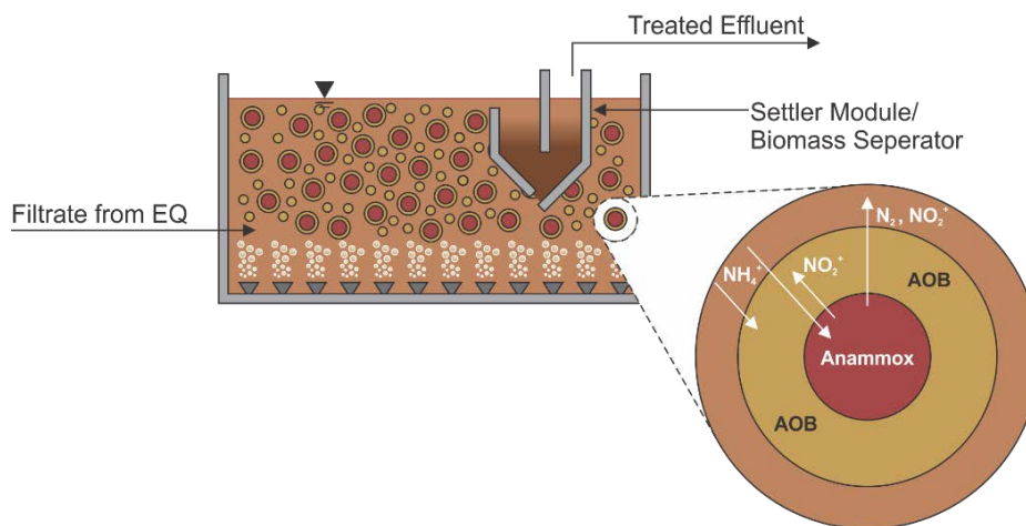
Figure 10.3-7: AnammoPAQ™ Upflow Granular Process and Theoretical Diffusion Patterns
