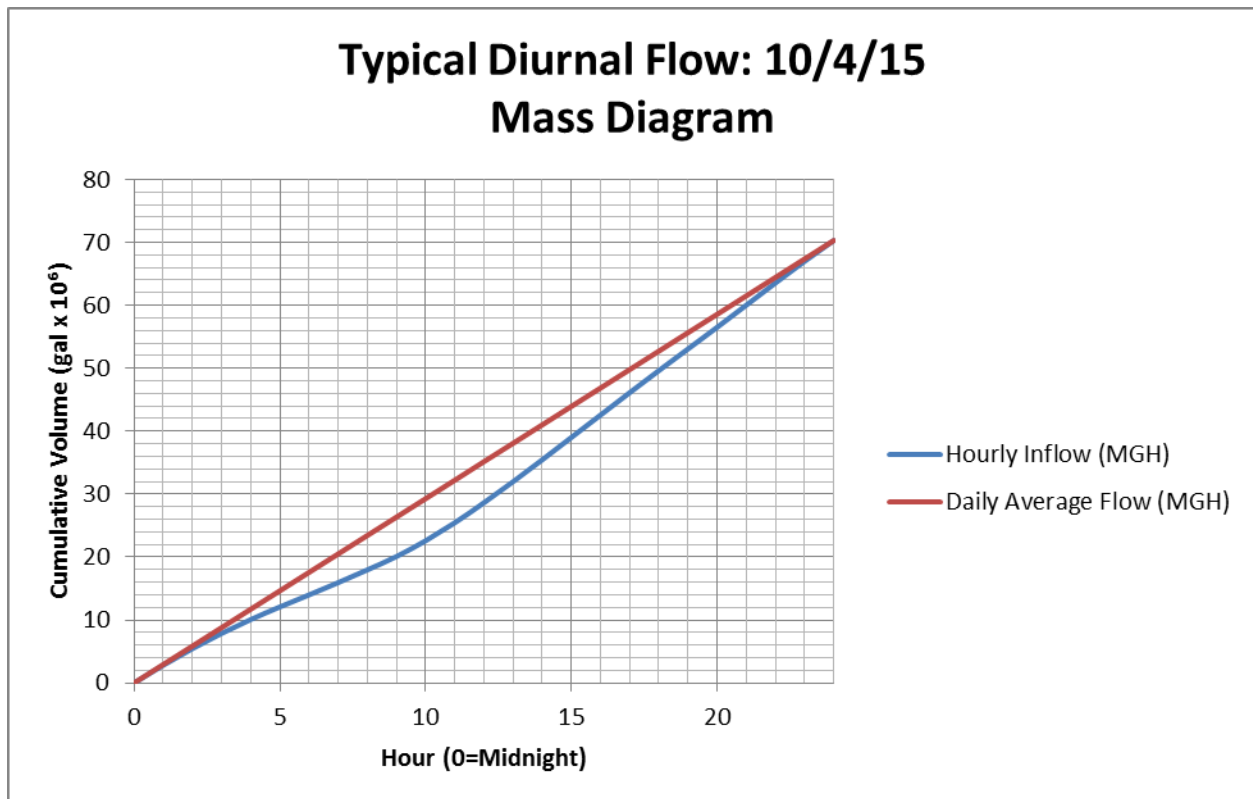
Figure 4.2-5: October 4, 2015 Mass Diagram
