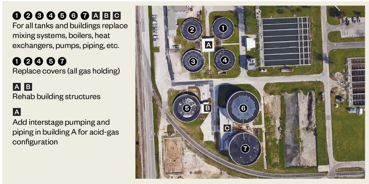
Figure 11.3-6: Site Plan – Proposed AGMD Facilities
