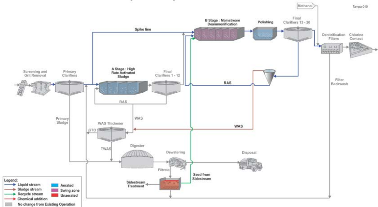
Figure 7.1-12: Alternative 4A– Next Generation Nitrogen Removal in Series
