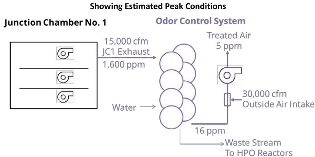
Figure 5.2-9: Flow Diagram of Alternative 2 Biotrickling Filters
