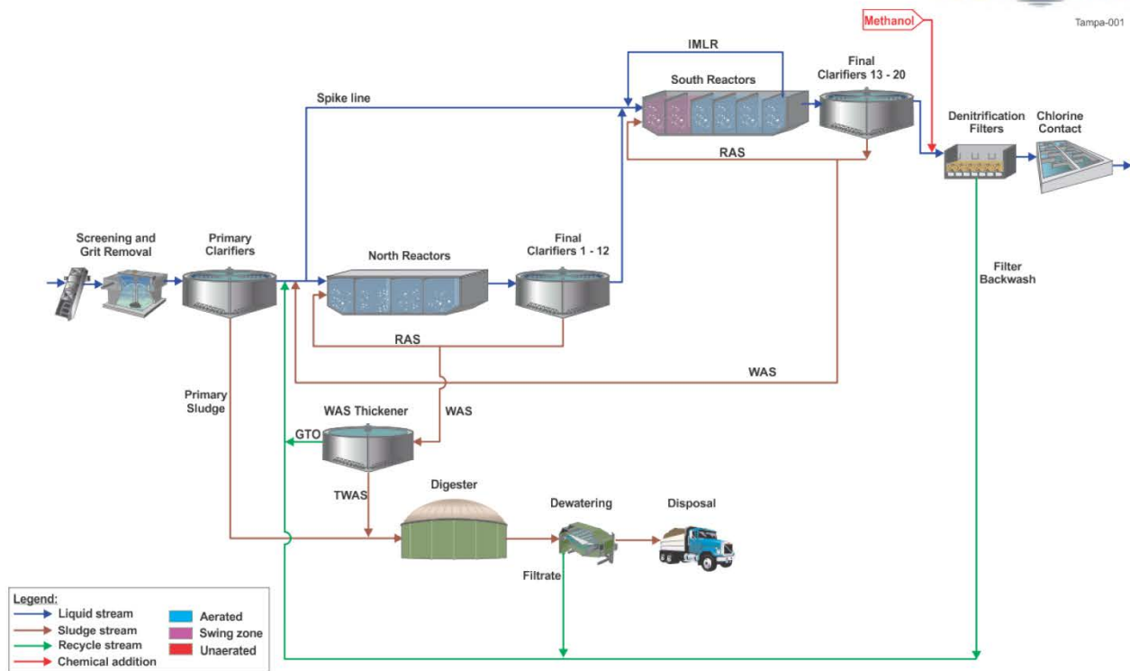
Figure 7.1-1: Existing HFC AWTP Process Schematic
