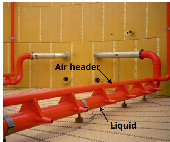
Figure 5.1-5: Example Jet Aeration System by MTS
