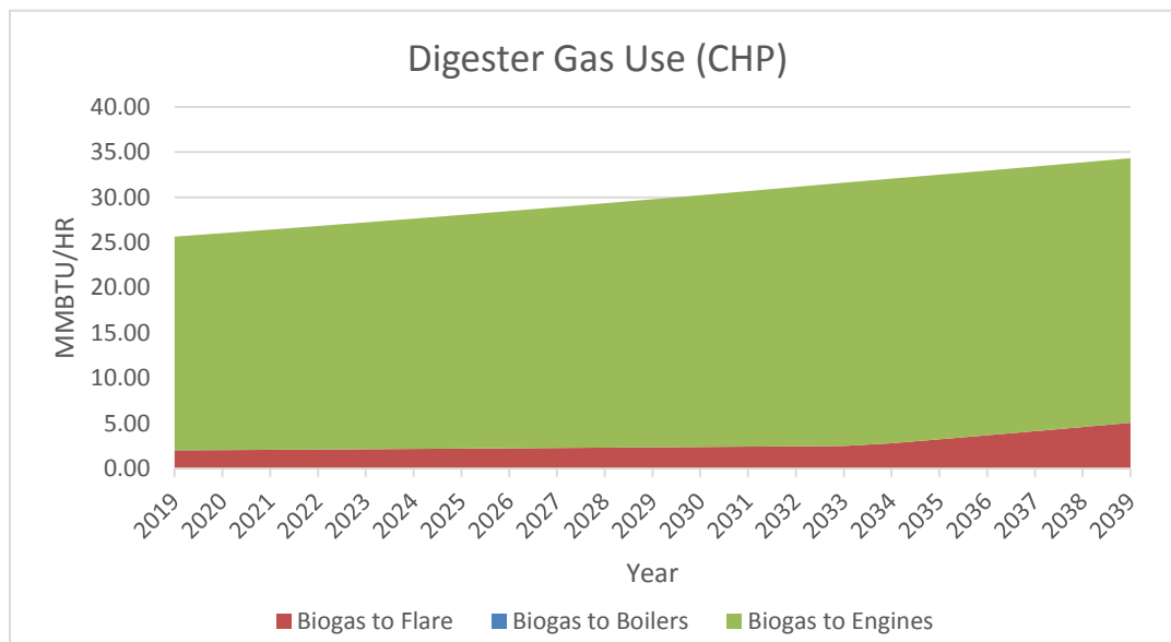
Figure 12.4-2: CHP Digester Gas Utilization (Optimize Existing Liquid Stream, Acid Gas Biosolids)
