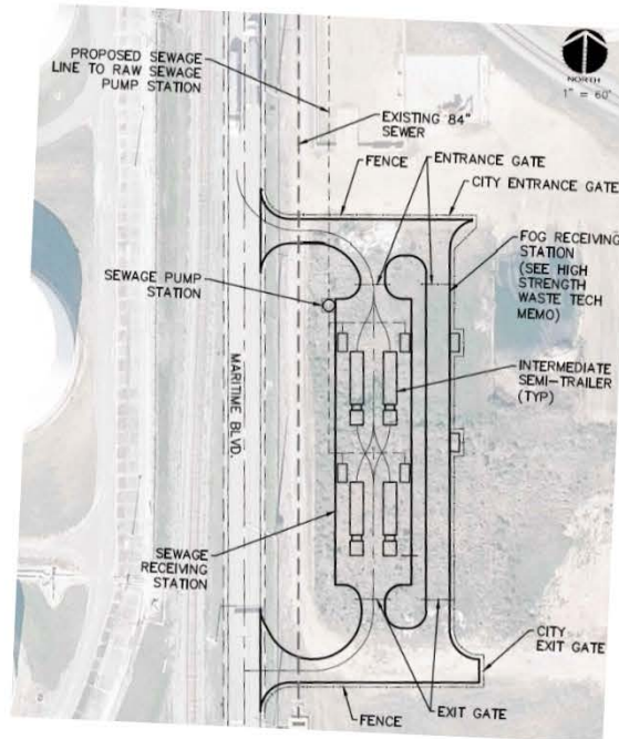
Figure ES.2-2: Proposed Sewage Receiving Station Layout
