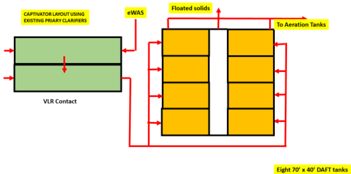
Figure 6.2-7: Captivator Process
