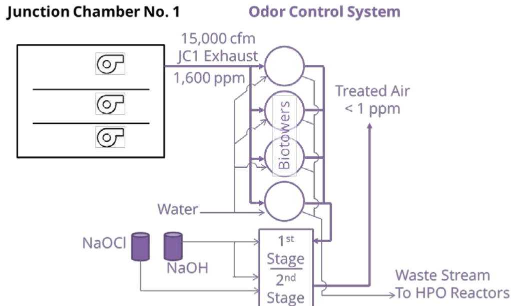
Figure 5.2-10: Flow Diagram of Alternative 3 Hybrid
