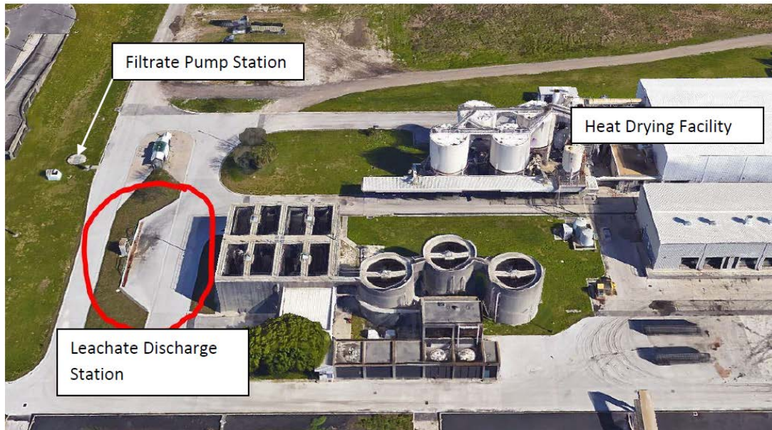
Figure 5.5-2: Aerial of Existing Leachate Discharge Station
