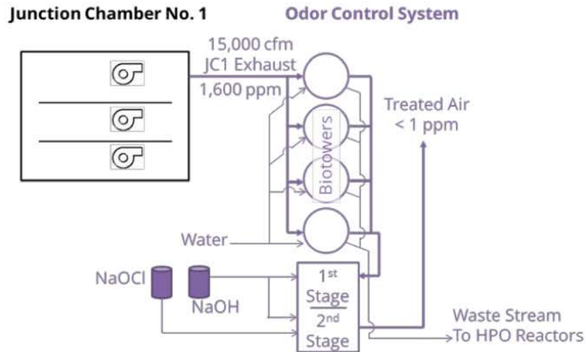
Figure ES.2-1: Flow Diagram of Hybrid Odor Control System
