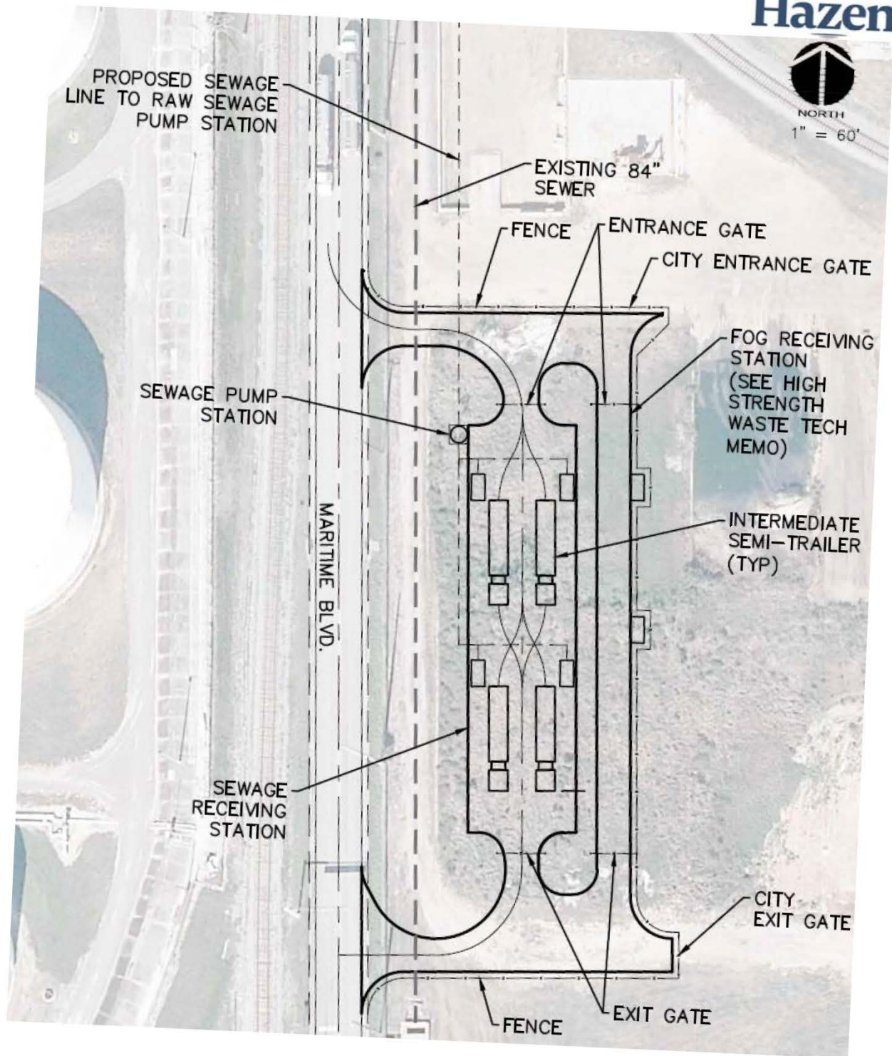
Figure 5.5-5: Proposed Sewage Receiving Station Layout
