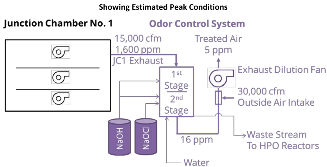
Figure 5.2-8: Flow Diagram of Alternative 1 – Chemical Scrubbing System
