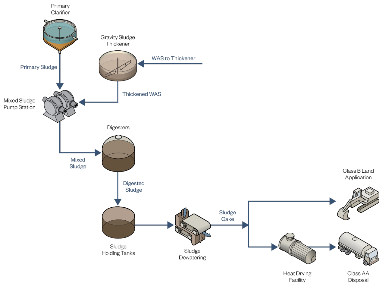
FIGURE ES.2-8: Existing HFC AWTP Process Schematic
