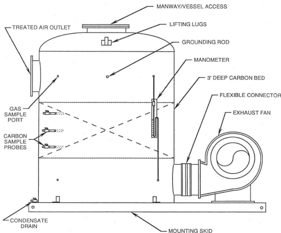
Figure 5.2-4: Schematic of a Typical Deep-Bed Carbon Asorber
