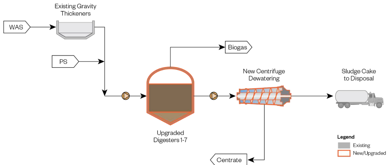
Figure 11.3-1: Solids Process Flow Schematic – Baseline Mesophilic Anaerobic Digestion
