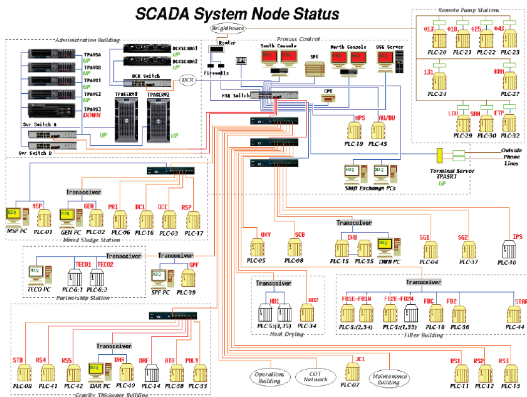
Figure 16.2-5: HFC AWTP Fiber Optic & Off-Site Communications Network
