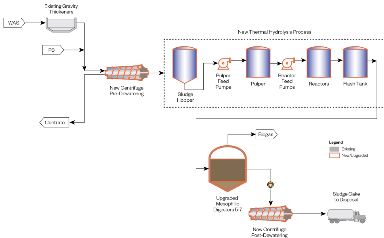
Figure 11.3-7: Solids Process Flow Schematic – Proposed THP Anaerobic Digestion Facilities
