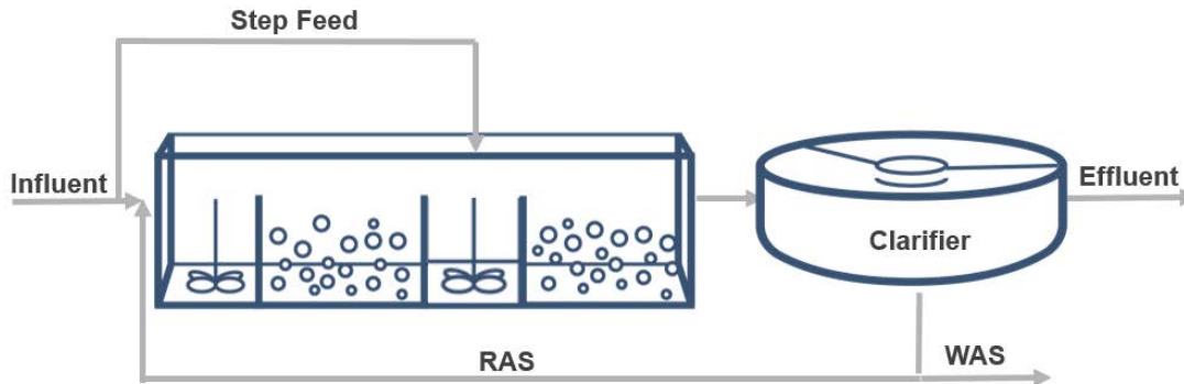
Figure 7.1-4: Step Feed Configuration
