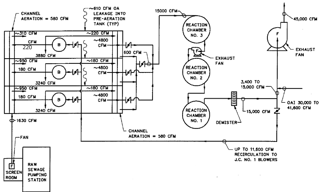
Figure 5.2-2: Existing Odor Control System Flow Diagram
