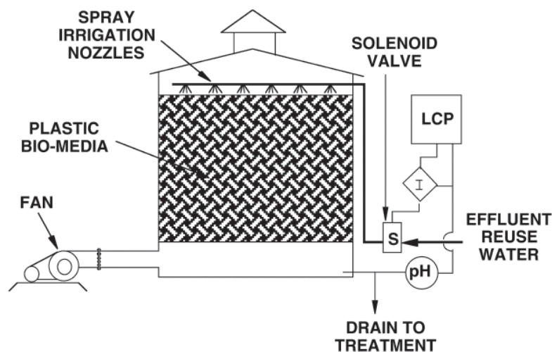
Figure 5.2-6: Schematic of a Typical Biotrickling Filter
