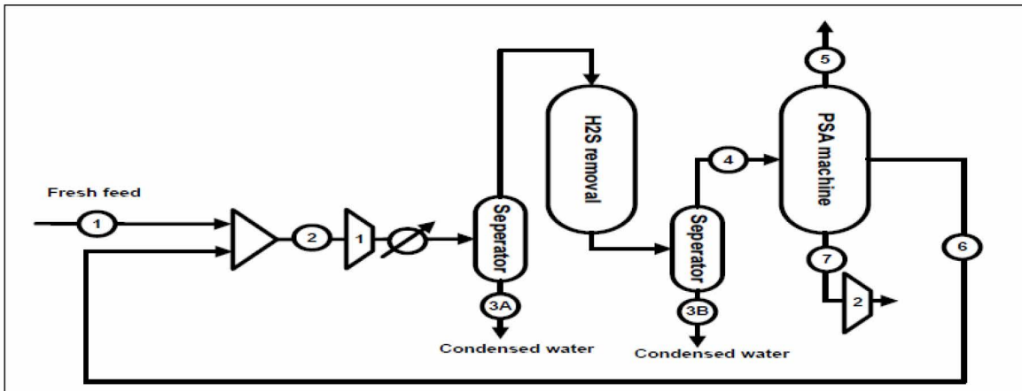
Figure 12.4-5: Typical Membrane Process Flow Diagram (Courtesy of Xebec)
