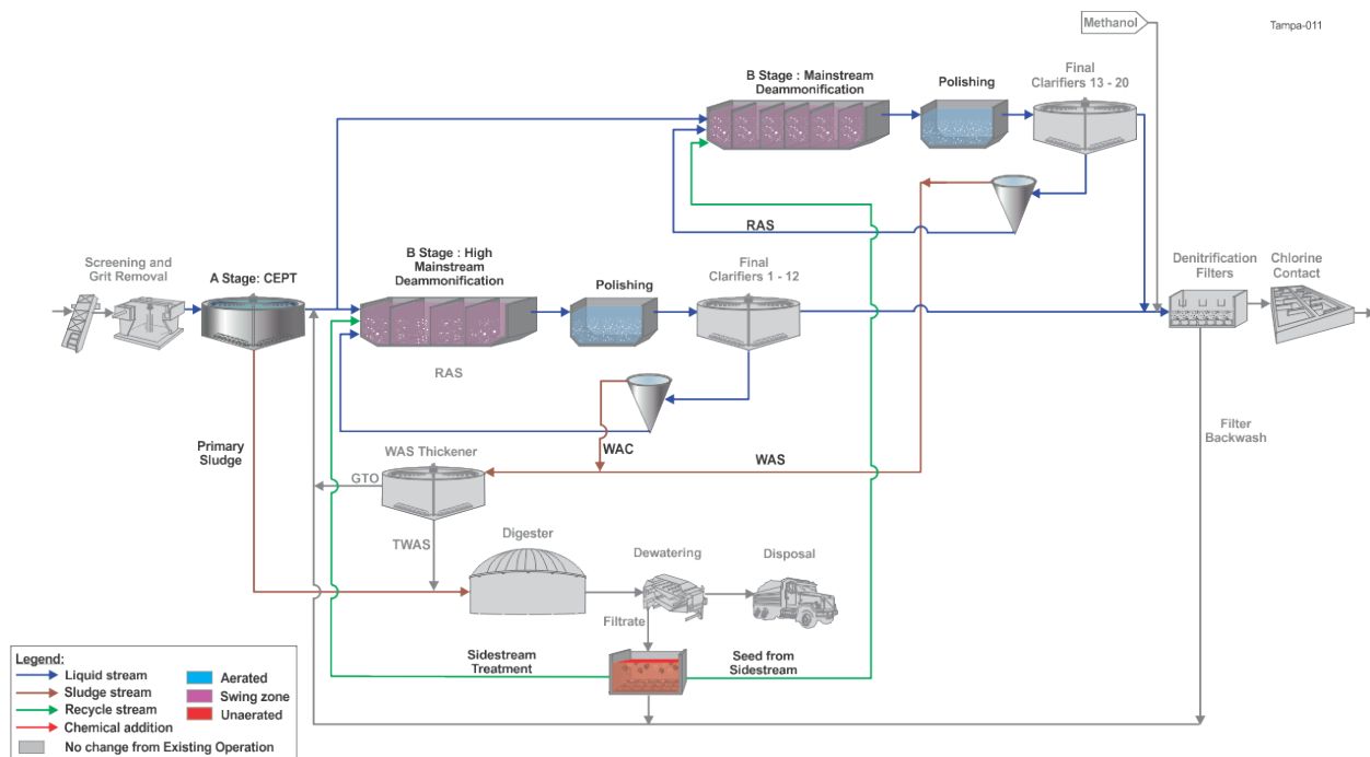
Figure 7.1-13: Alternative 4B – Next Generation Nitrogen Removal in Parallel
