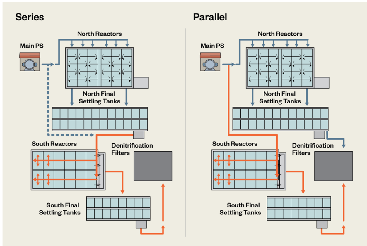
Figure 7.1-5: Stage Operation: Series vs. Parallel
