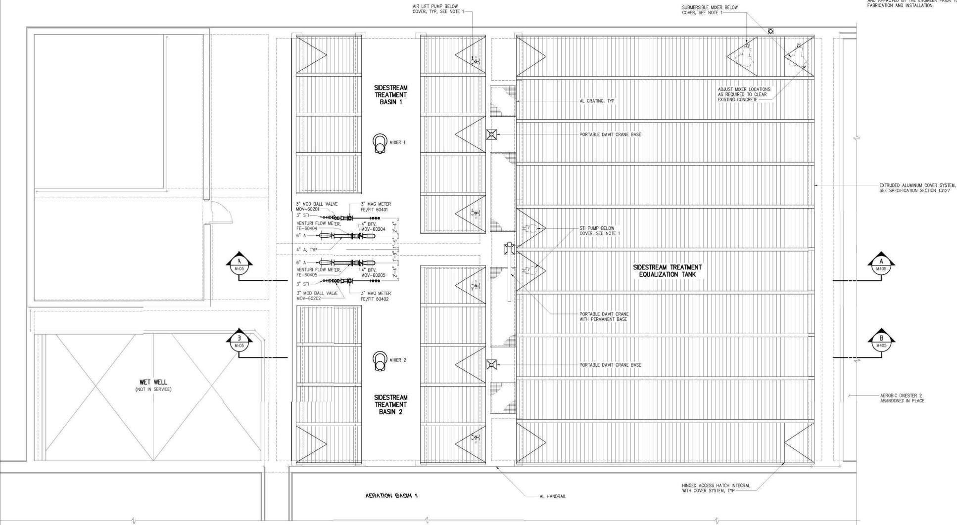
TOP PLAN 1/4" = 1'-0"
