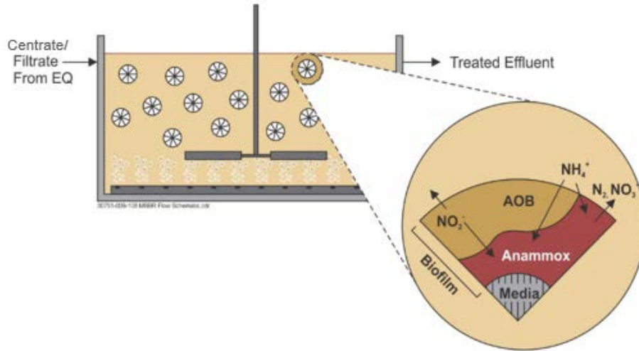
Figure 10.3-5: ANITA™ Mox (MBBR) Biofilm Configuration and Theoretical Diffusion Patterns. Note that Anammox in the figure is used to reference AnAOB.
