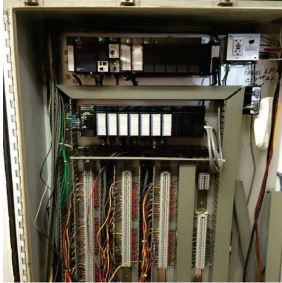
Figure 16.2-3: PLC-15 GE PACSystems RX3i PLC with GE 90-30 Remote I/O
