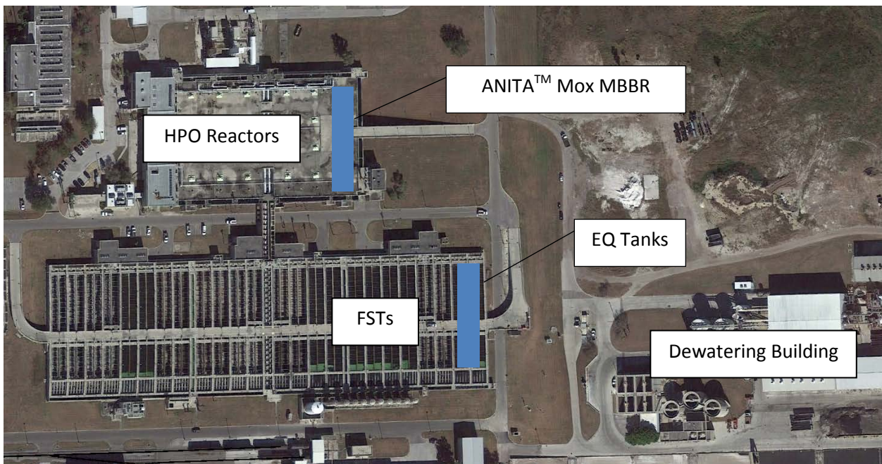
Figure 10.4-1: Proposed Location for ANITA™ Mox MBBR and EQ Tank
