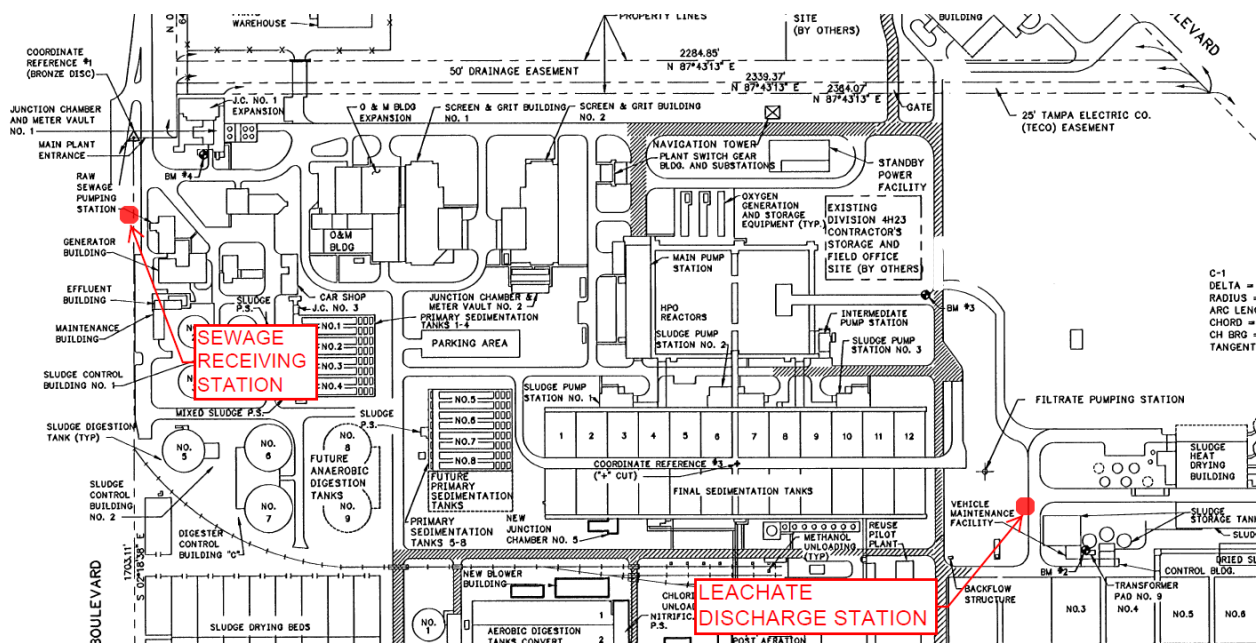
Figure 5.5-3: Existing Location of Industrial Waste Stations at HFC AWTP
