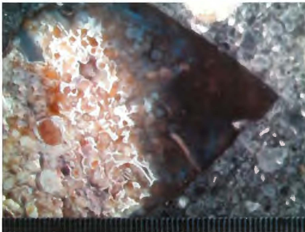
Photo 11 – Magnified view of chert found in sample. Scale = 0.01 inches
