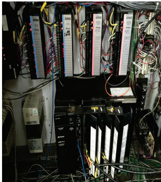
Figure 16.2-4: PLC-5:33 GE 90-70 PLC with GE Genius I/O
