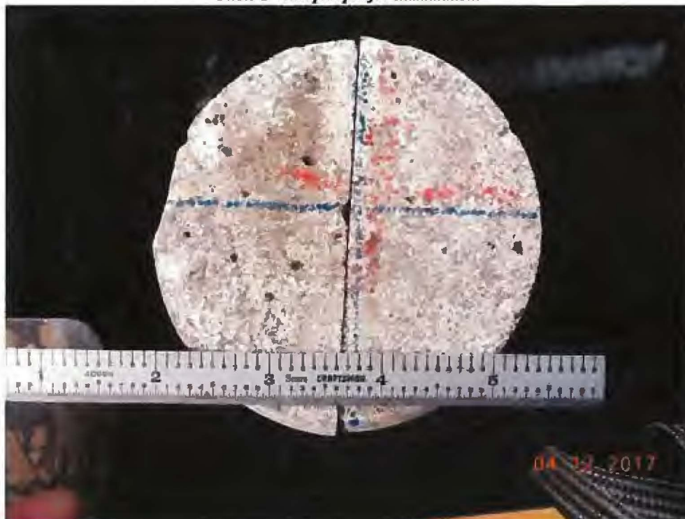
Photo 3 – Outer surface of core sample.
