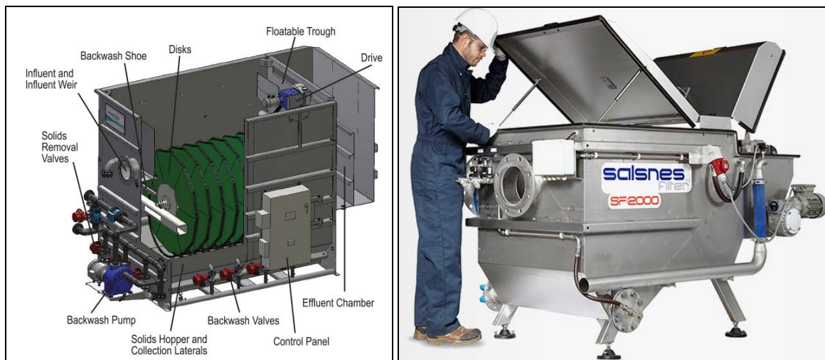
Figure 6.2-4: Primary Filter (Left Picture: AquaPrime; Right Picture: Salsnes)
