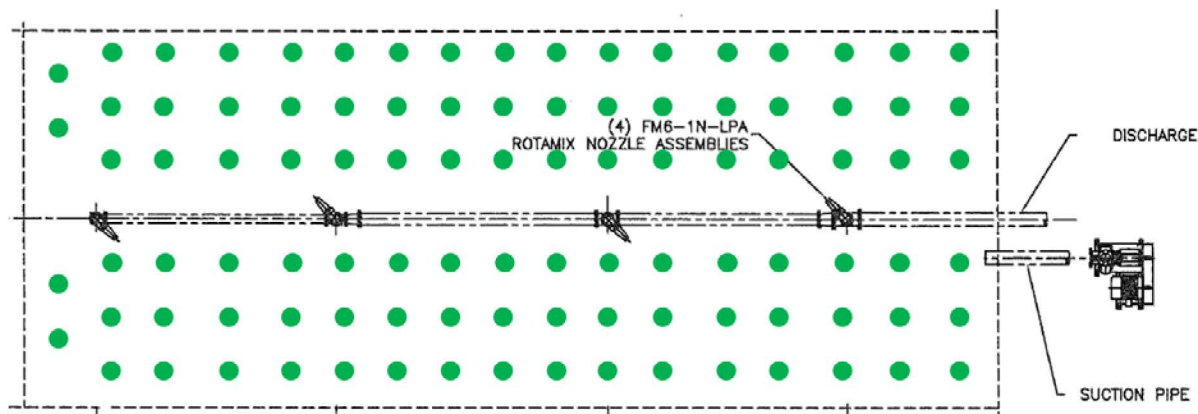
Figure 5.1-8: Proposed Layout for Alternative 3
