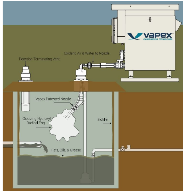
Figure 5.2-7: Diagram of a Hydroxyl Radical Oxidation System
