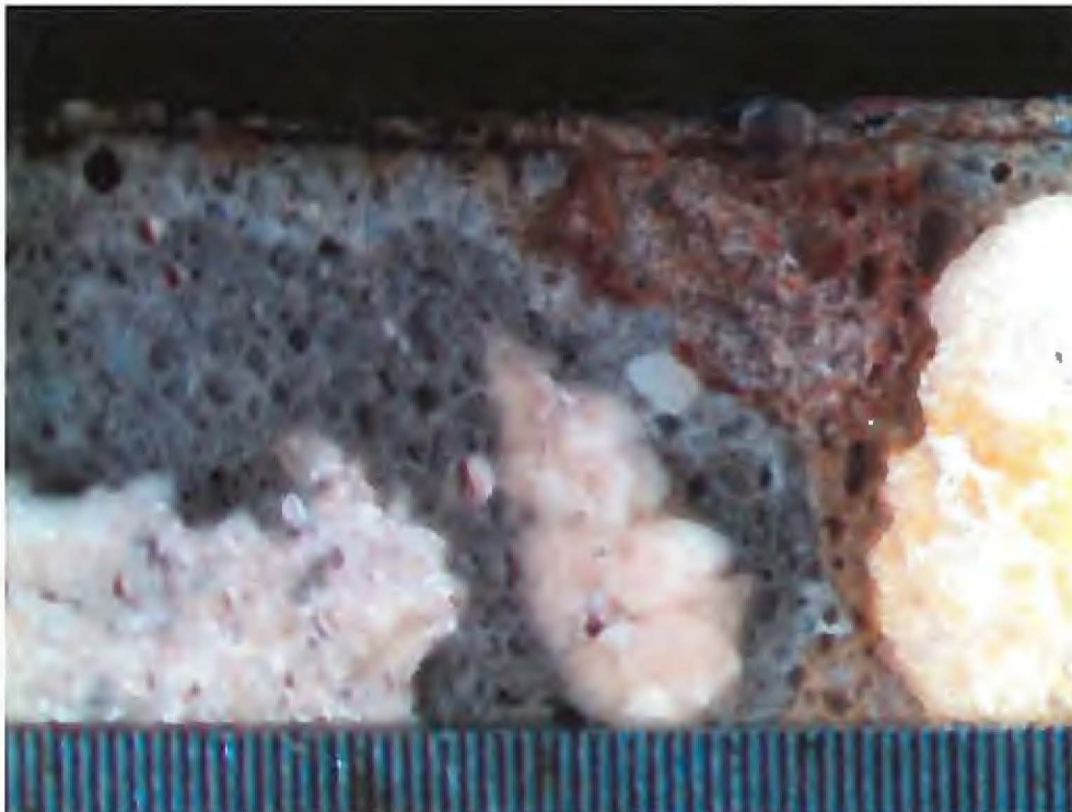
Photo 7 – Close-up view of larger stain inclusion (Struvite crystals) at surface. Scale = 0.01 inches
