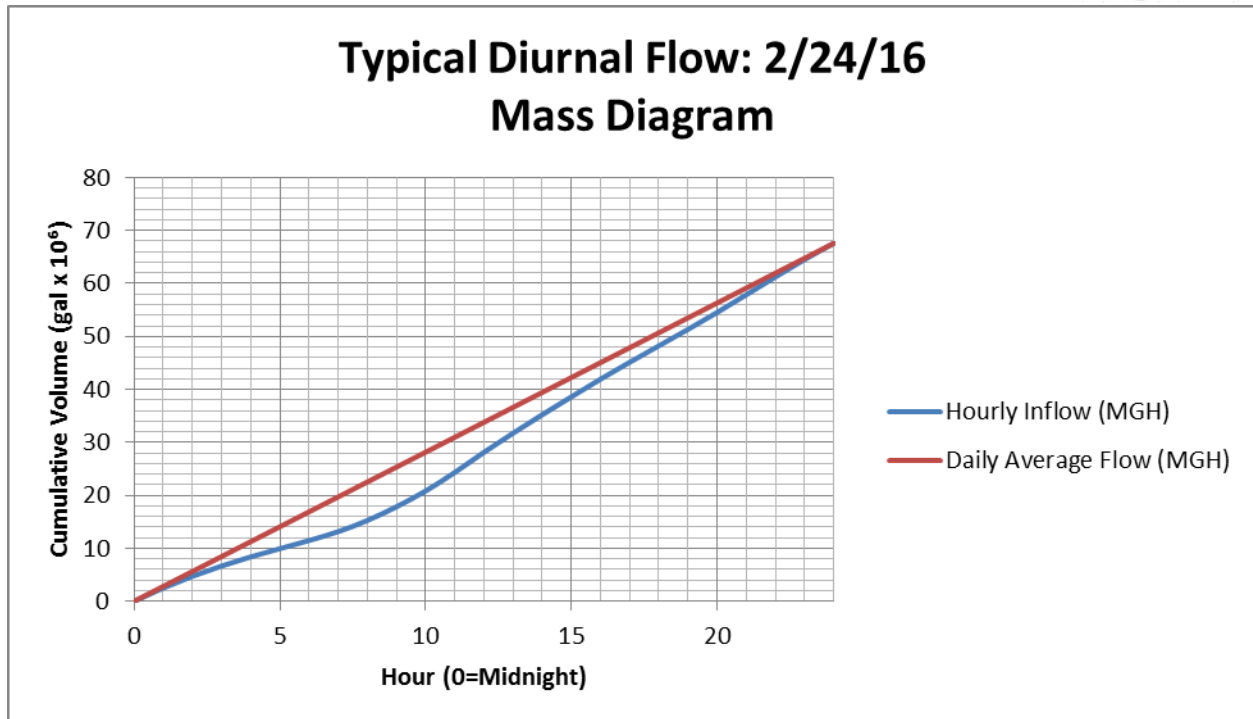
Figure 4.2-4: February 24, 2016 Mass Diagram
