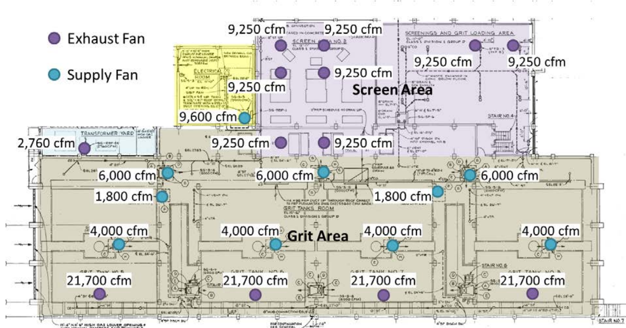
Figure 5.3-2: Existing Ventilation in S&G Building No. 1
