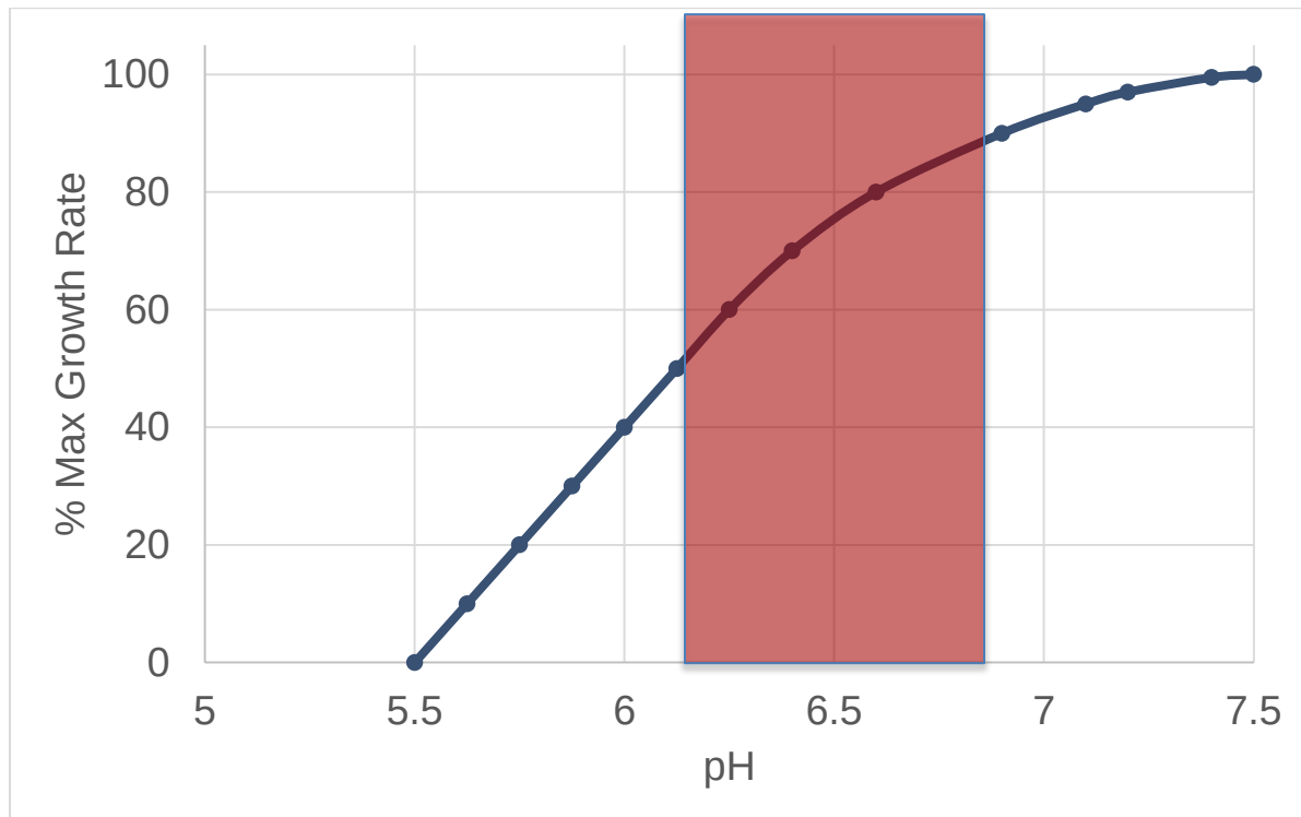
Figure 7.3-1: Correlation Between pH and Maximum Growth Rates of Nitrifying Bacteria
