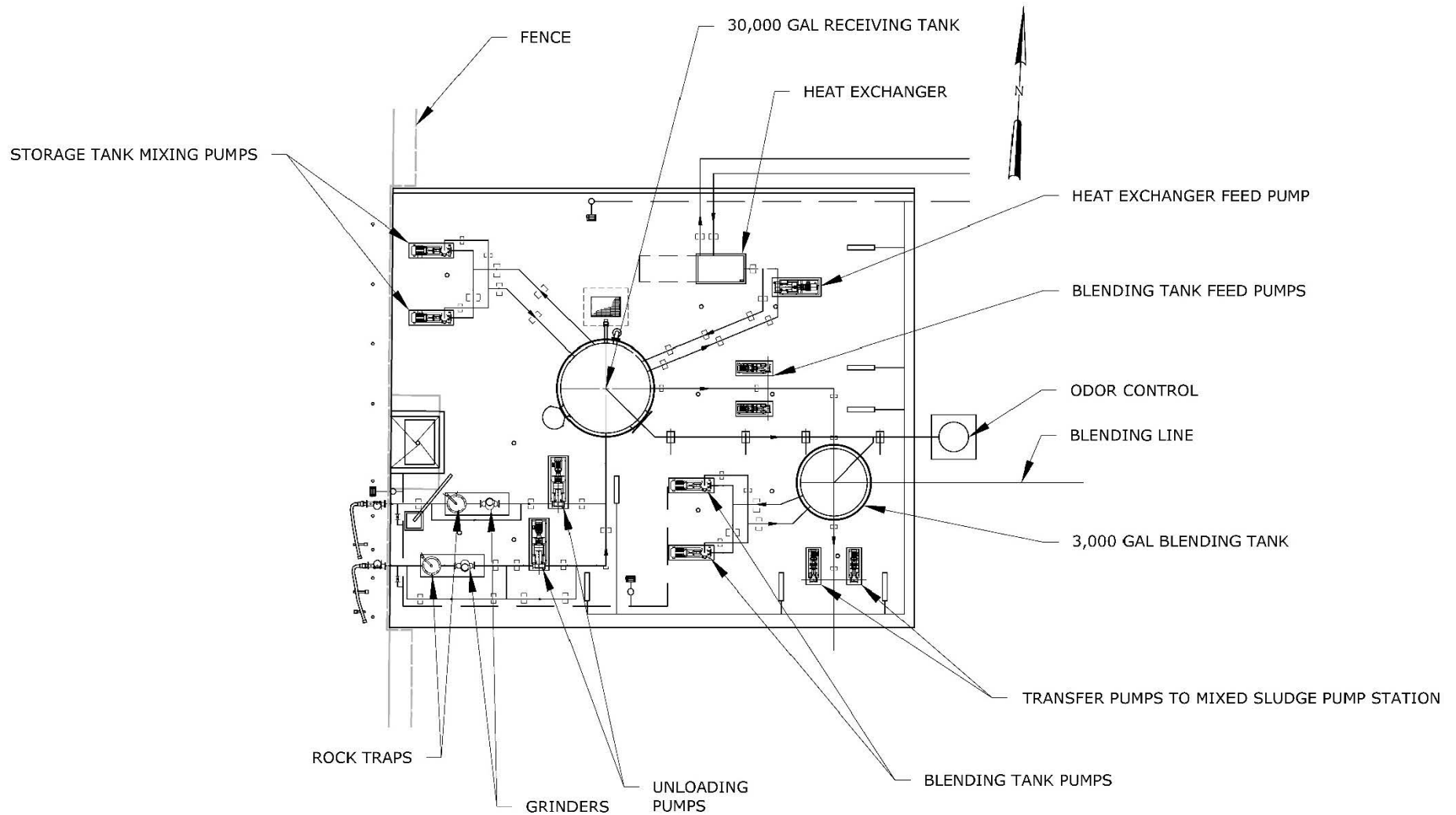
Figure 13.6-3: Potential Layout of HSW Receiving Station
