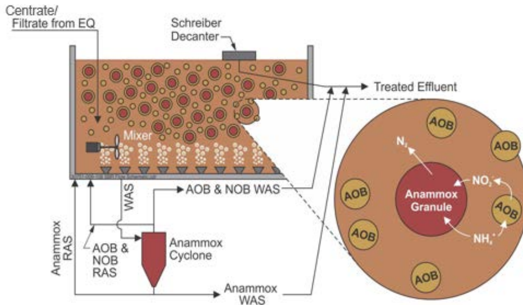
Figure 10.3-3: DEMON® SBR Schematic. Note that Anammox in the figure is used to reference AnAOB.
