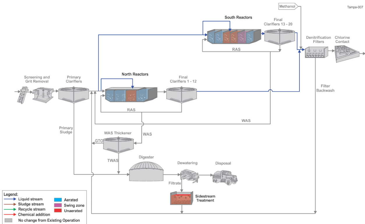
Figure 7.1-11: Alternative 3B – Step Feed in Parallel
