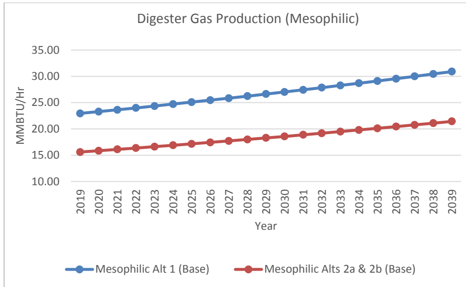
Figure 12.3-1: Mesophilic Biosolids Treatment Digester Gas Production
