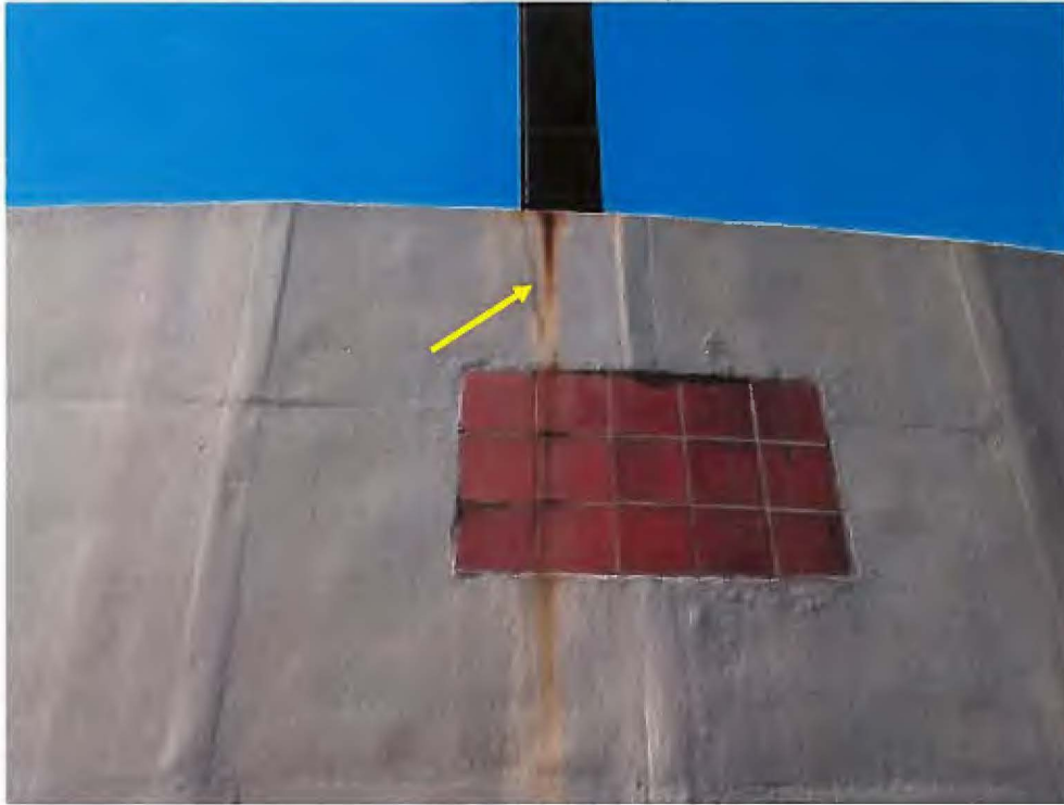
Photo 23 – North external wall of tank with vertical cracks.
