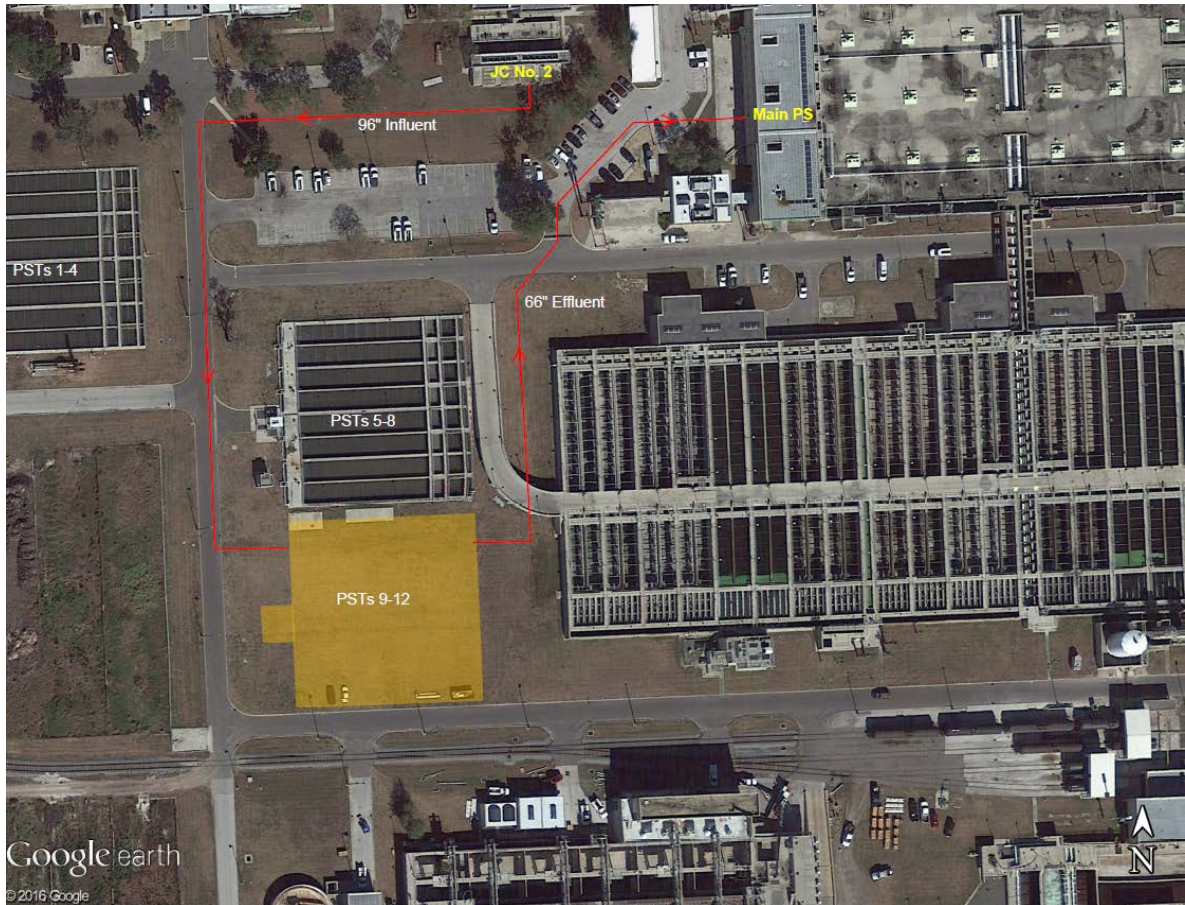
Figure 6.2-3: Additional PST Area of Construction
