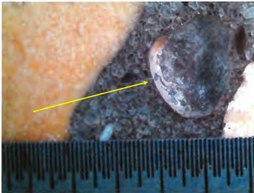
Photo 9 – Magnified view of entrapped air void. Scale = 0.01 inches
