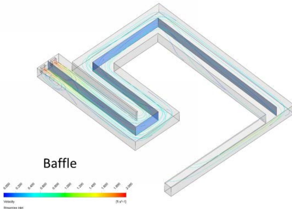
Figure ES.2-6: CFD Modeling with Proposed CCT Center Baffle Wall
