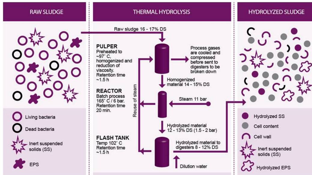
Figure 11.3-8: CAMBI's Thermal Hydrolysis Process ( www.cambi.no )
