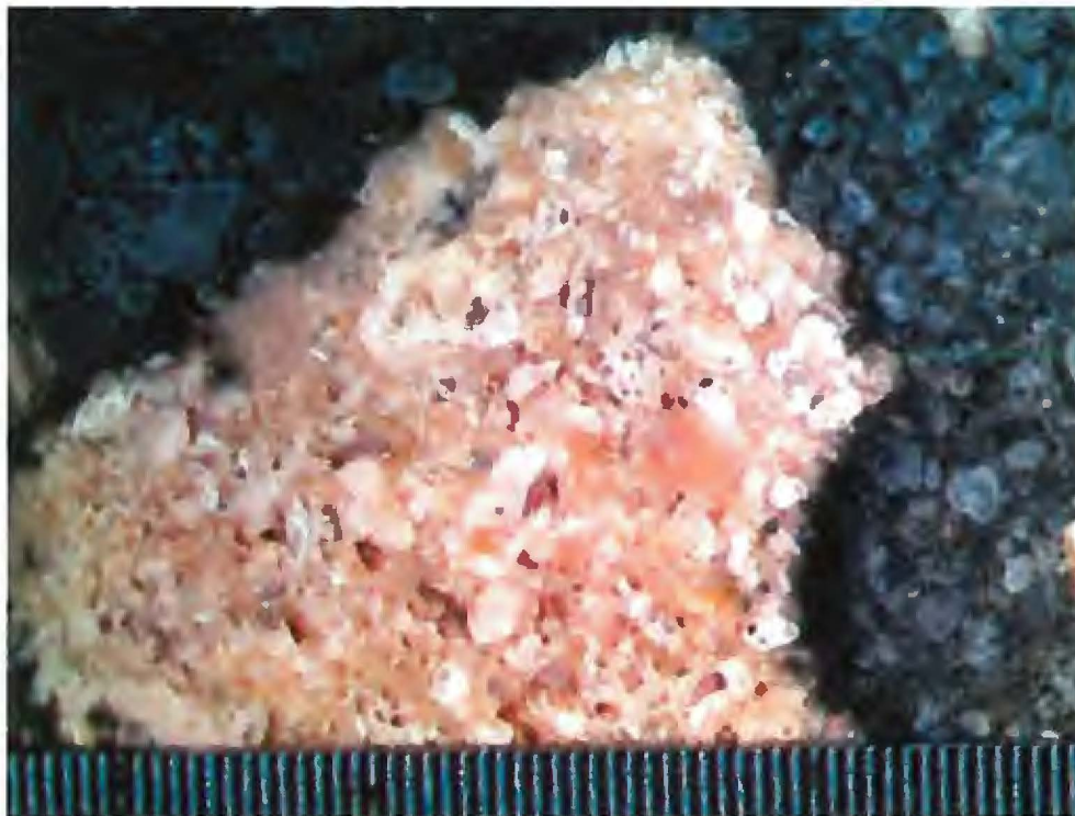
Photo 12 – Magnified view of aggregate piece with partial ring/halo indicating possible aggregate reaction. Scale = 0.01 inches
