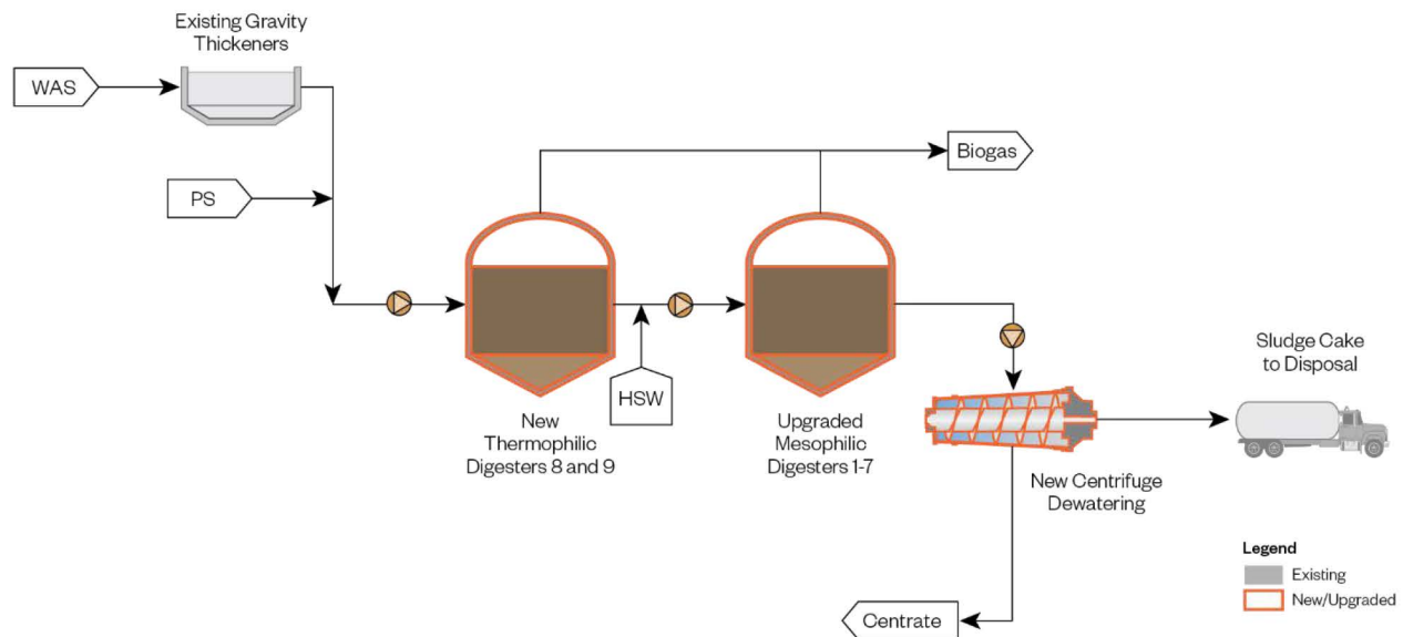
Figure 11.3-3: Solids Process Flow Schematic – Temperature-Phased Anaerobic Digestion
