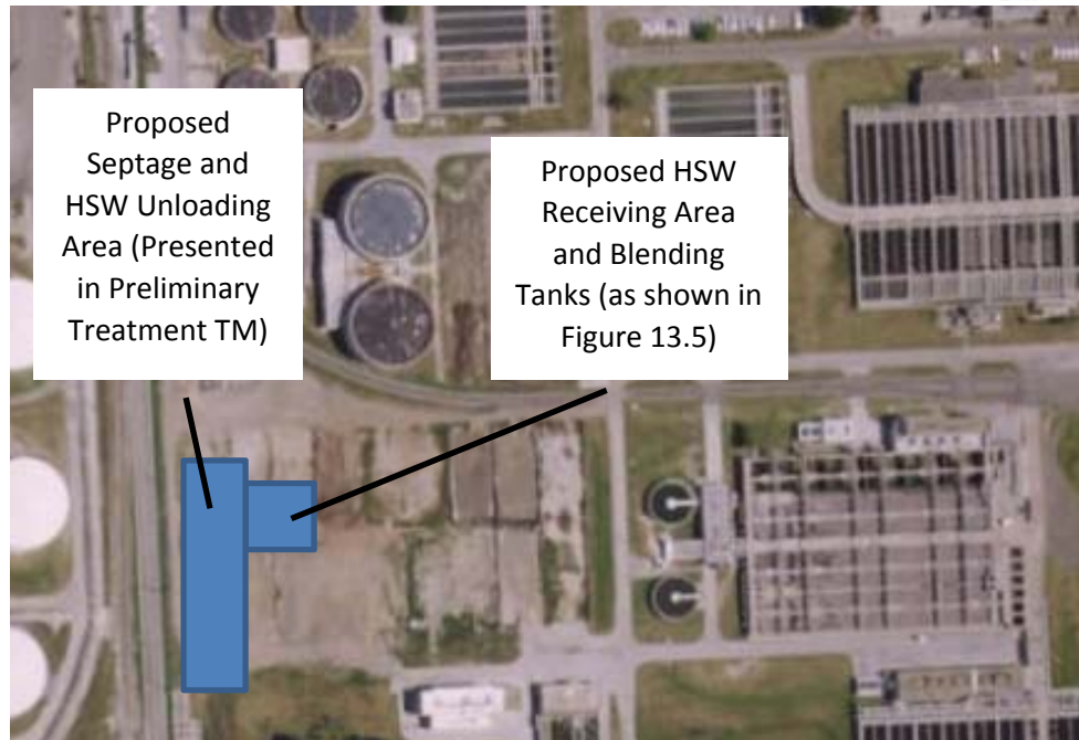
Figure 13.6-2: Proposed Location of the HSW Unloading Area and Receiving Station
