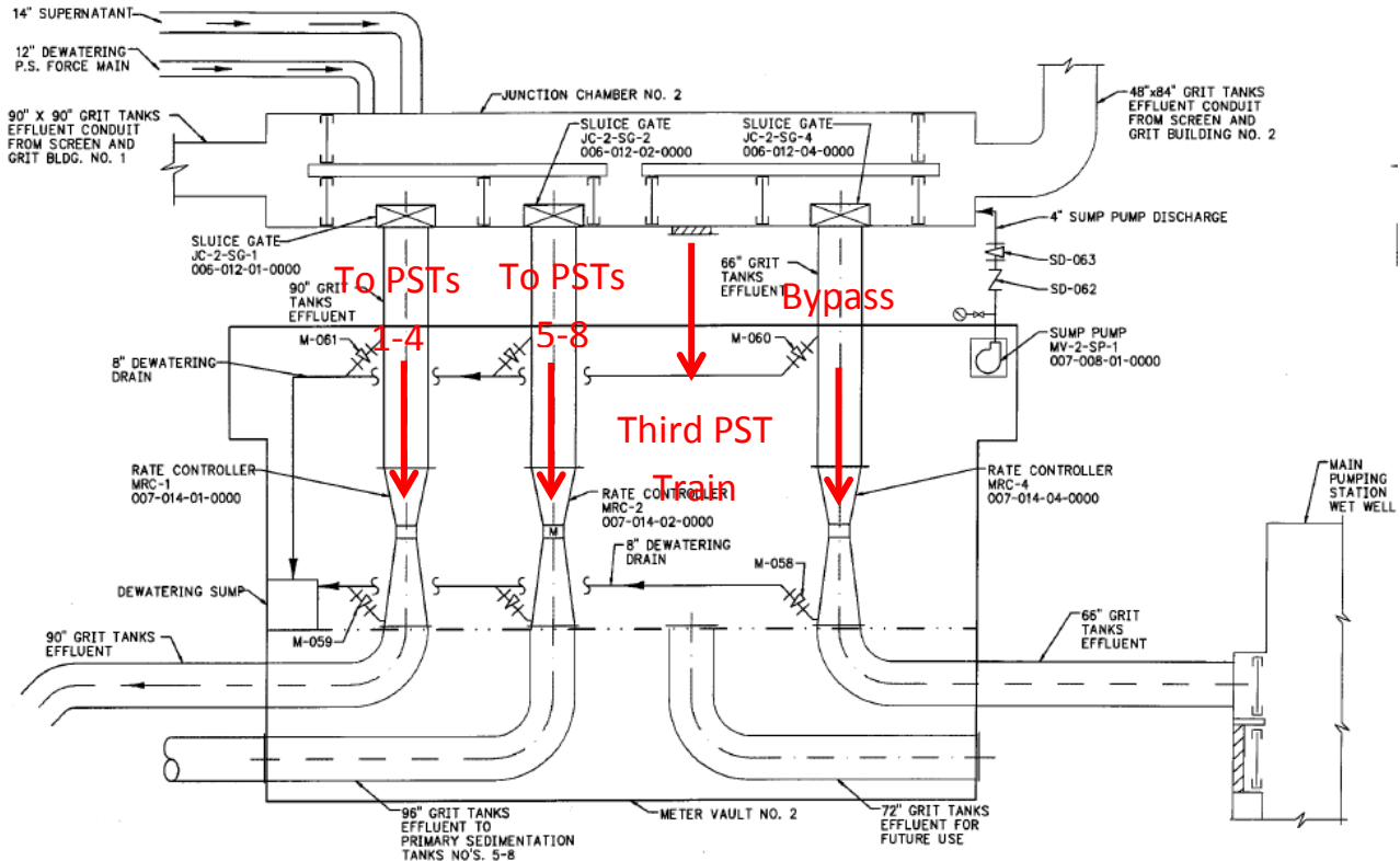
Figure 6.2-2: Junction Chamber No. 2 Diagram
