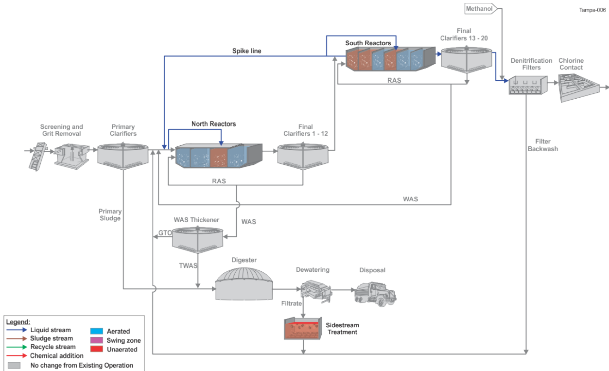
Figure 7.1-10: Alternative 3A – Step Feed in Series
