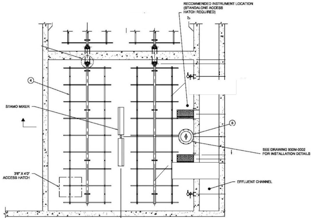
Figure 10.4-2: Plan View of ANITA™ Mox MBBR System
