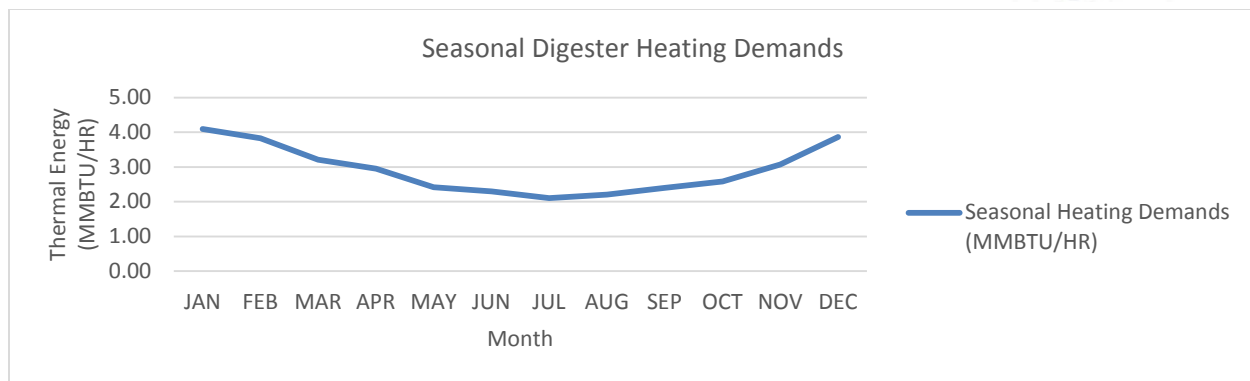
Figure 12.2-1: Seasonal Digester Heating Demands
