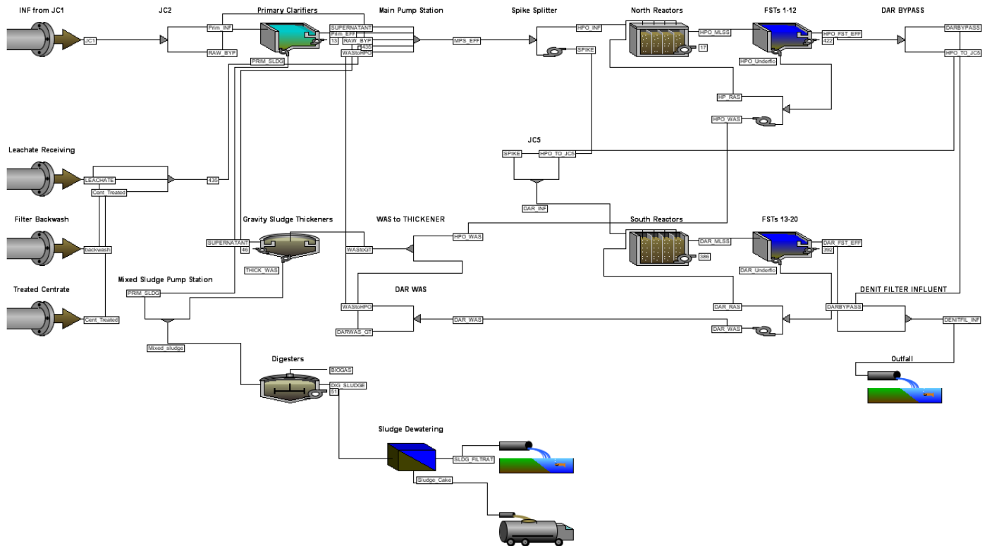
Figure 7.2-2: GPS-X® Layout for BNR Process Evaluation
