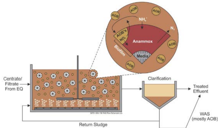
Figure 10.3-6: ANITA™ Mox (IFAS) Biofilm Configuration and Theoretical Diffusion Patterns. Note that Anammox in the figure is used to reference AnAOB.
