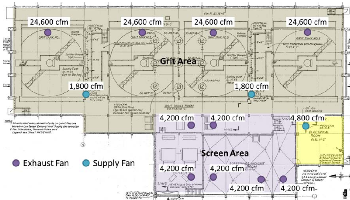
Figure 5.3-3: Existing Ventilation in S&G Building No. 2
