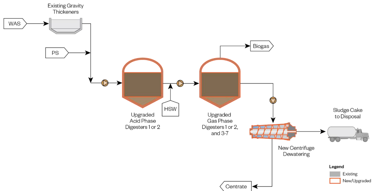
Figure 11.3-5: Solids Process Flow Schematic – Proposed AGMD Facilities
