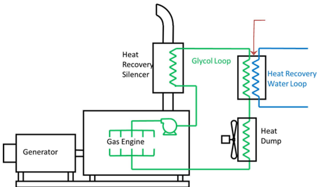
Figure 12.4-1: CHP Process Diagram
