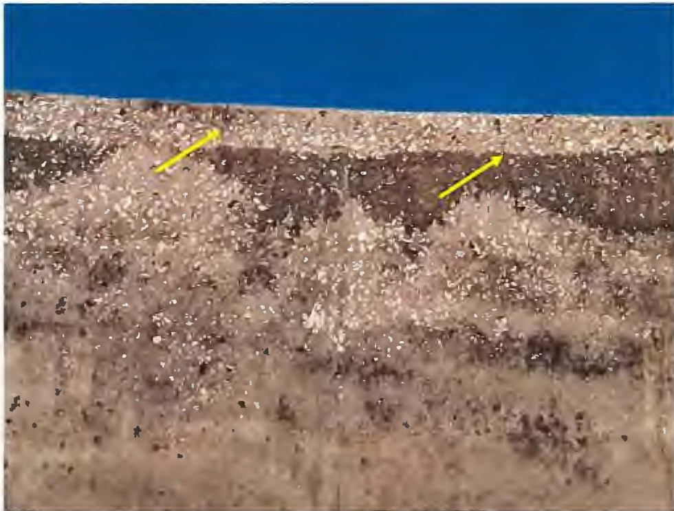
Photo 22 – Northwest wall of tank with vertical cracks.
