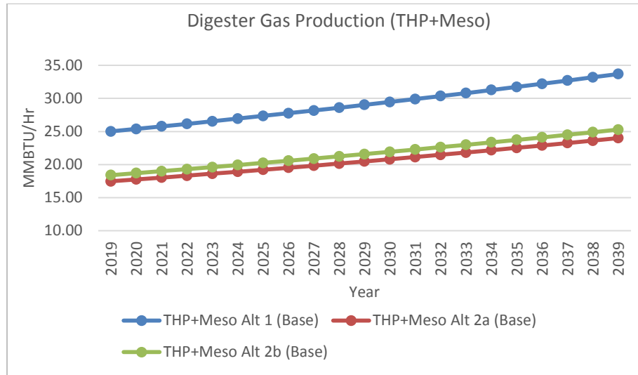
Figure 12.3-3: THP+Meso Biosolids Treatment Digester Gas Production
