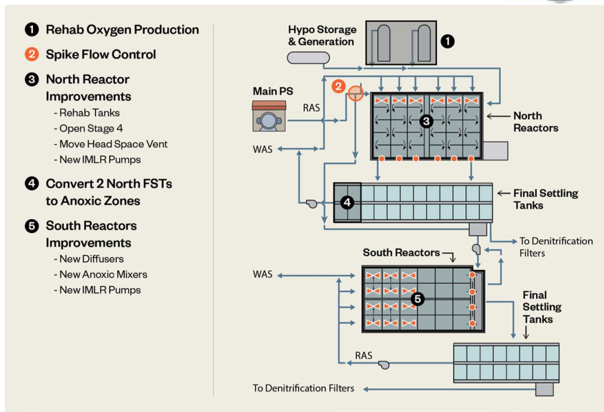
Figure 7.4-2: Summary of Capital Improvements Req. for Alternative 2H-MLE In Parallel (Keep HPO)
