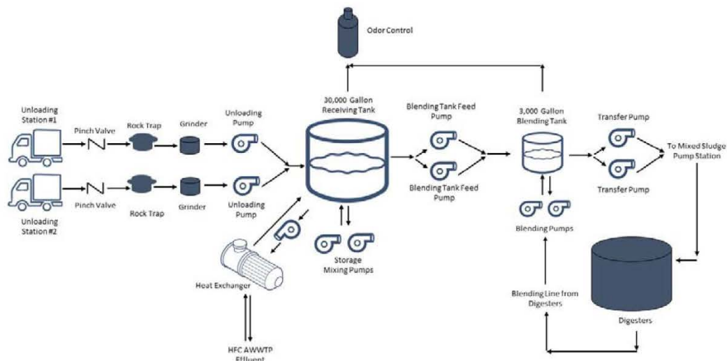
Figure 13.6-1: Potential Schematic of HSW Receiving Station
