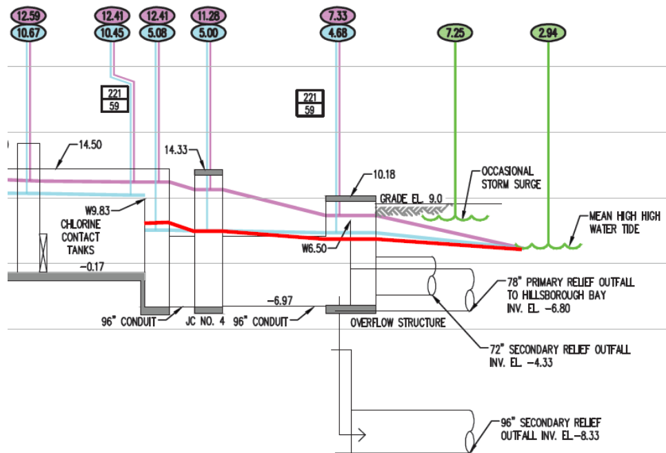
Figure 9.6-3: Combined Hydraulic Model Improvements
