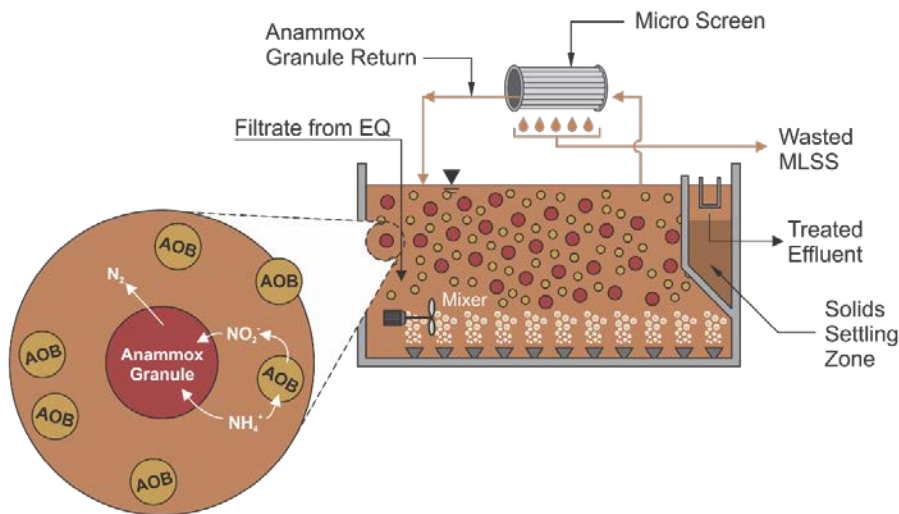
Figure 10.3-4: DEMON® Continuous Flow Schematic. Note that Anammox in the figure is used to reference AnAOB.
