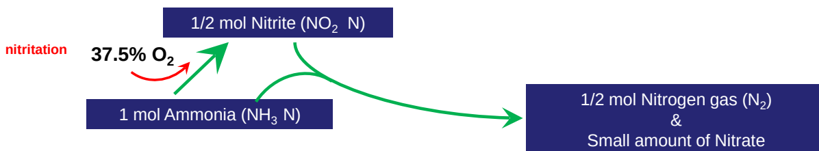
Figure 10.3-1: Deammonification Pathway for Nitrogen Removal
